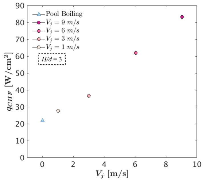
Figure 4. Critical heat flux (CHF) for the jet impingement (corresponding to V_j = 1 m/s, 3 m/s, 6 m/s, and 9 m/s; H/d = 3 ) and pool boiling configurations.
