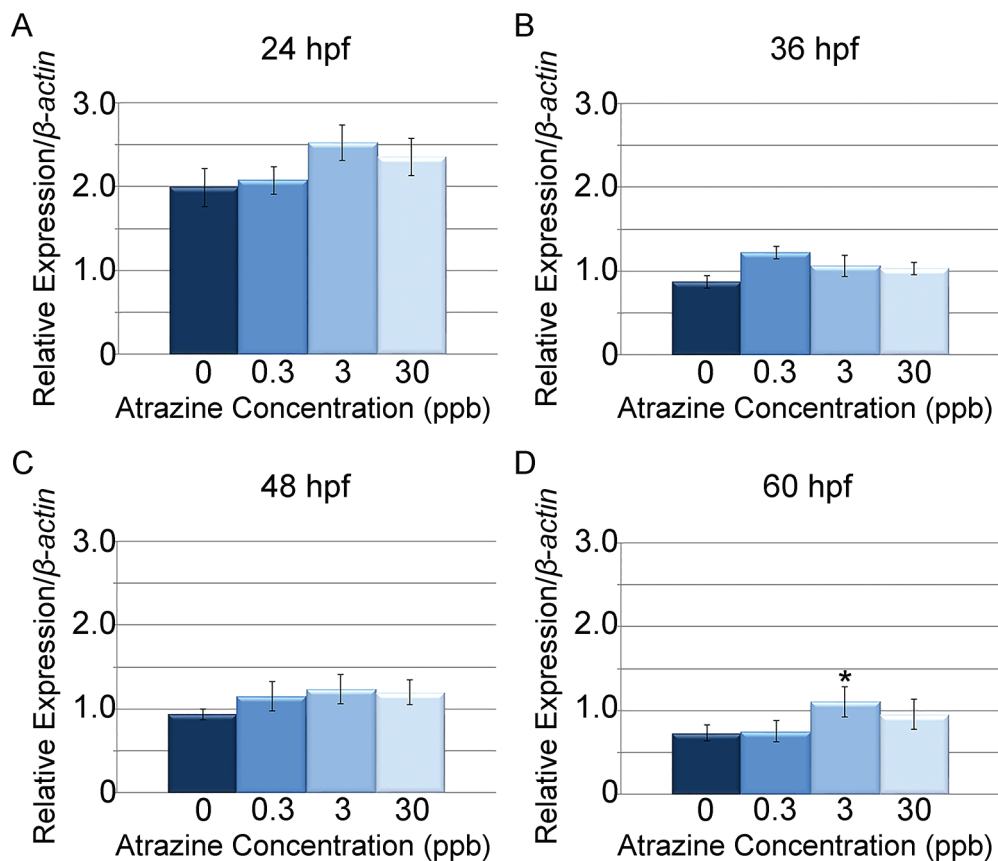
The time course of ttc3 relative expression after developmental atrazine exposure. No significant differences in relative expression were observed between treatment groups at 24 hpf (A), 36 hpf (B), or at 48 hpf (C). At 60 hpf, the 3 ppb treatment had increased relative expression as compared to the controls (D). n = 6, qPCR run in triplicate, error bars represent standard deviation, * = p < 0.05. (hpf: hours post-fertilization)
