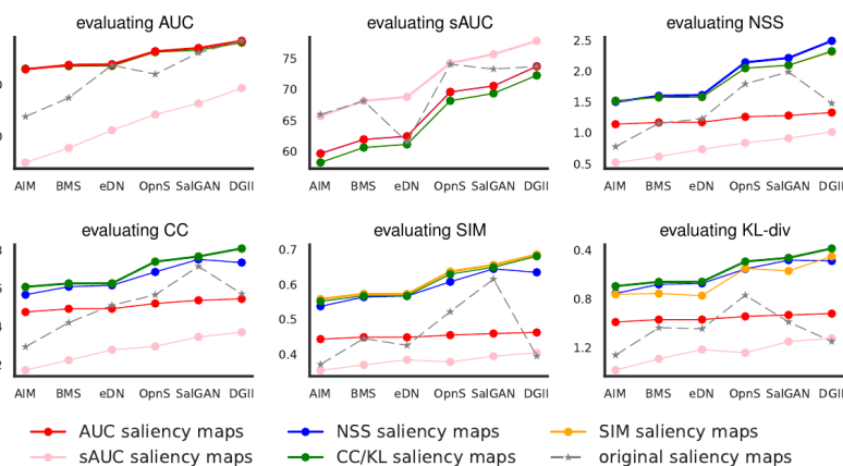
Figure 2: Evaluation on the MIT1003 dataset: The correct saliency map for each metric (thick lines) results in the best possible performance among all saliency map types (other lines) for each model and results in consistent model rankings across metrics – unlike the original saliency maps (dashed lines)
