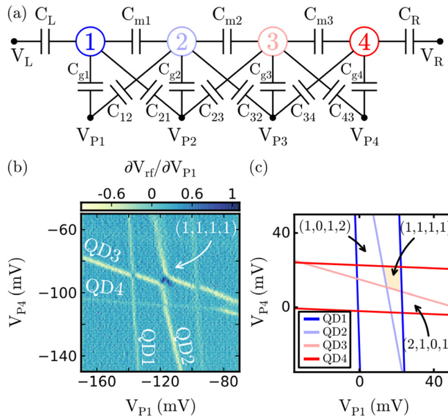
FIG. 2. (a) Schematic of the QD capacitive model used throughout this paper to calculate the charge stability diagrams. (b) Charge stability diagram close-up of the (1,1,1,1) region, in the plane defined by plunger gates P 1 and P 4 , with V_{P2} = -40 mV and V_{P3} = -180 mV. (c) Calculated transition lines using the model of (a) and C_{gi} = C_{mi} = C_L = C_R = 10 aF and C_{i\pm 1,i} = 1 aF for i = 1, 2, 3, 4 .
