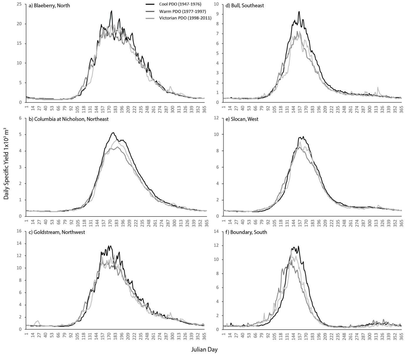
211 Figure 2. Annual hydrographs for streams with the longest record in each of the 6 Canadian Columbia 212 Basin sub-regions. Values represent daily means through the three main north Pacific regime shifts, the 213 cool phase from 1947 to 1976, the subsequent warm phase from 1977 to 1997, and the Victorian Mode 214 from 998 to 2011.
