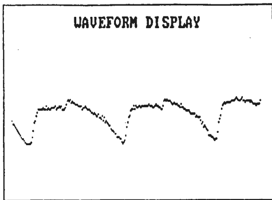
Figure 14 ADULT LX WAVEFORM /a/ VOCAL FRY
