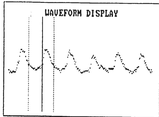
Figure 8 CHILD LX WAVEFORM /a/ QUASI-OPEN QUOTIENT = .55
