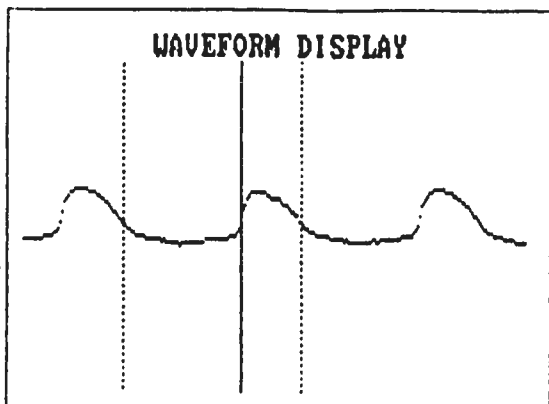
Figure 22 ADULT LX WAVEFORM /i/ BREATHY OQ = .66 MODAL OQ = .56
