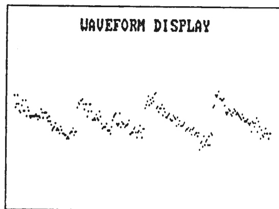
Figure 19 CHILD LX WAVEFORM /u/ VOCAL FRY
