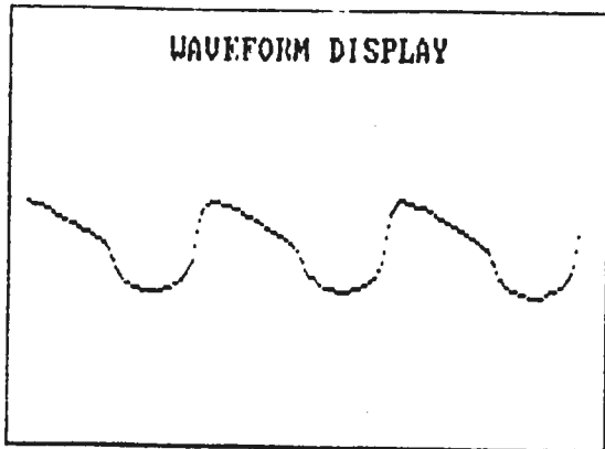
Figure 1 ADULT LX WAVEFORM /a/
