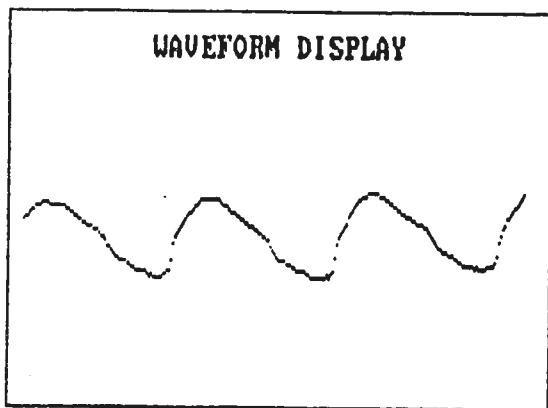
Figure 5 ADULT LX WAVEFORM /u/
