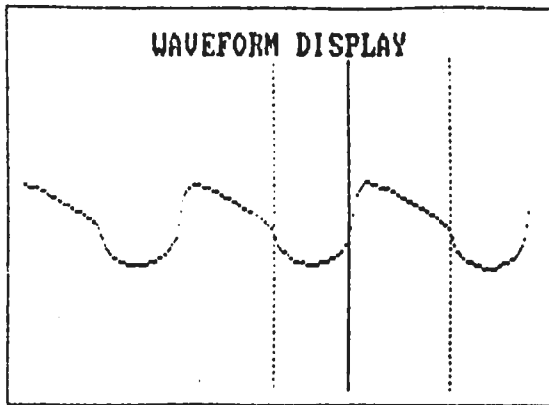
Figure 7 ADULT LX WAVEFORM /a/ QUASI-OPEN QUOTIENT = .43
