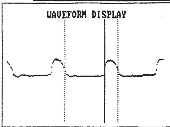
Figure 20 ADULT LX WAVEFORM /a/ BREATHY OQ = .75 MODAL OQ = .43
