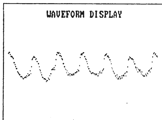
Figure 6 CHILD LX WAVEFORM /u/
