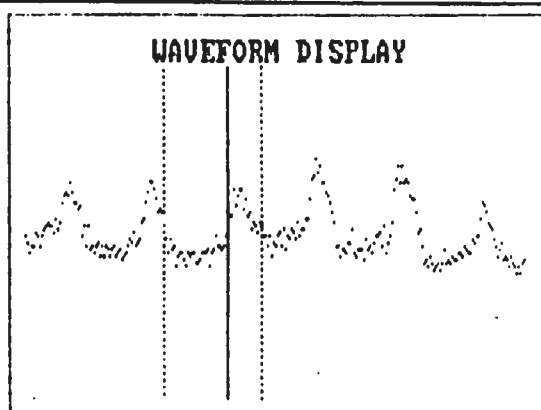
Figure 21 CHILD LX WAVEFORM /a/ BREATHY OQ = .65 MODAL OQ = .55
