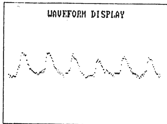
Figure 2 CHILD LX WAVEFORM /a/
