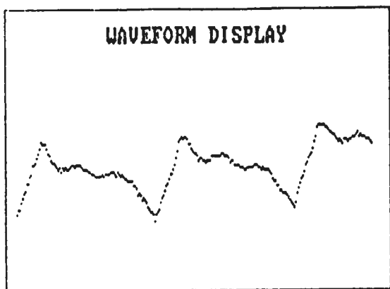
Figure 16 ADULT LX WAVEFORM /i/ VOCAL FRY
