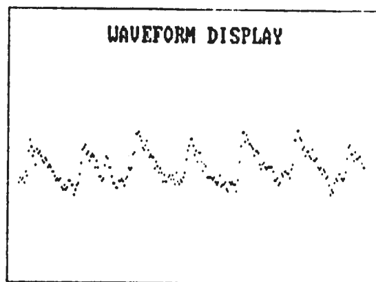
Figure 17 CHILD LX WAVEFORM */i/ VOCAL FRY
