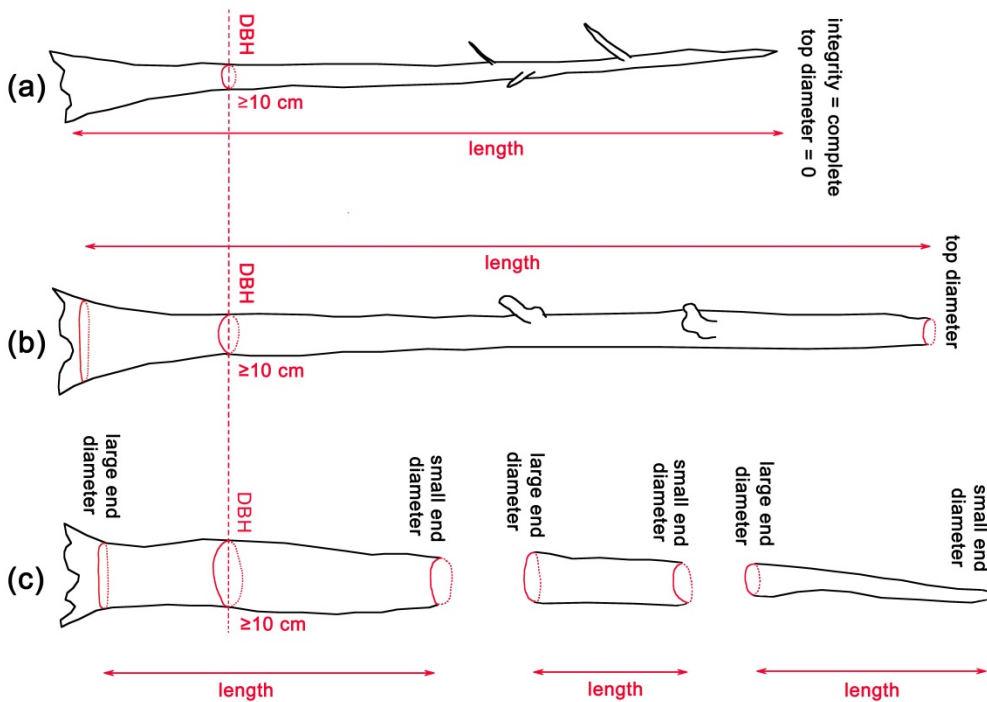
Fig. 4. Required measurements of logs for volume estimates of a complete log (a), incomplete log (b) and a log fragmented in pieces (c).
