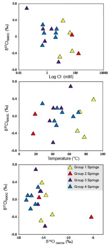
Figure A2. \delta^{37}\text{Cl} values from hot springs proximal and distal to the Cordillera Blanca detachment, as a function of log Cl - concentration (top), spring surface temperature (middle), and \delta^{18}\text{O} values (bottom). No obvious trends are observed.
