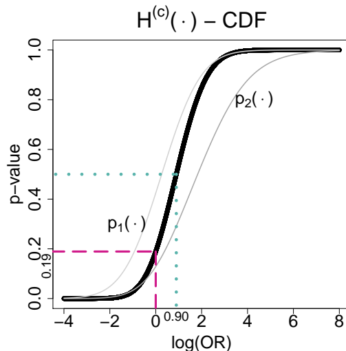
FIGURE 4.4: The combined p -value function of the two studies shown in Table 4.1 plotted as a CDF. The dotted teal line indicates the median of the combined p -value function. The dashed magenta line shows the p -value under the null value of 0.
