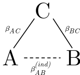
FIGURE 3.3: The graphical network on which the simulation study is based.
