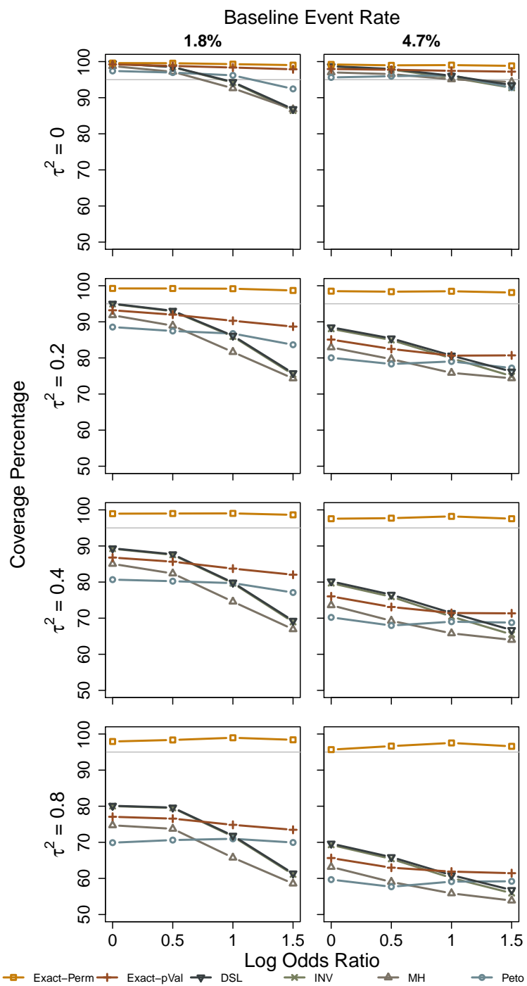
FIGURE 2.3: This figure compares the confidence interval coverage of several existing methods to our new exact method with varied values of \mu (baseline event rate), \tau^2 , and \theta (log odds ratio). The horizontal, grey line marks the nominal 95% coverage value.
