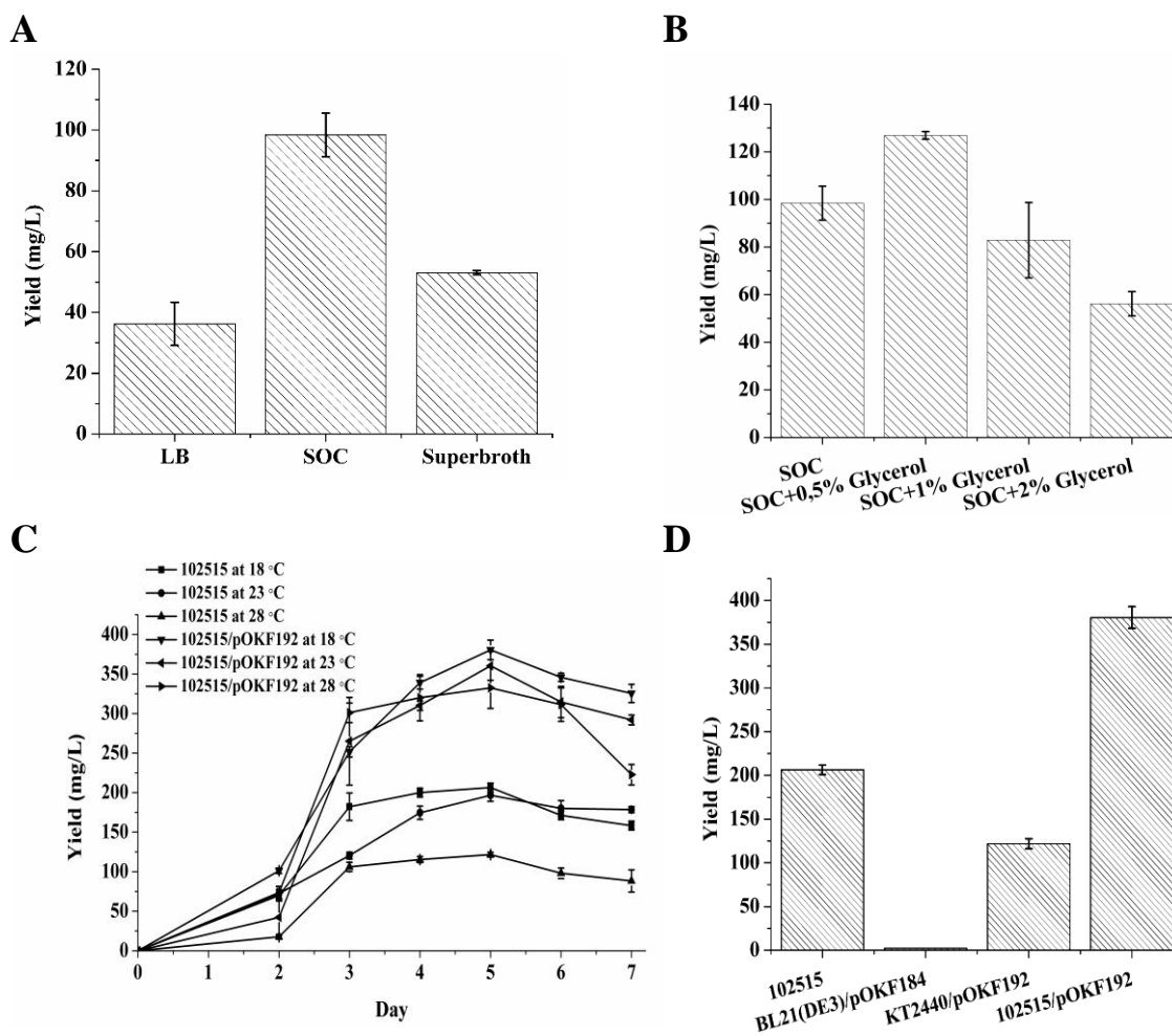
FIG. 18. Optimization of zeaxanthin diglucoside production in Pseudomonas sp.
