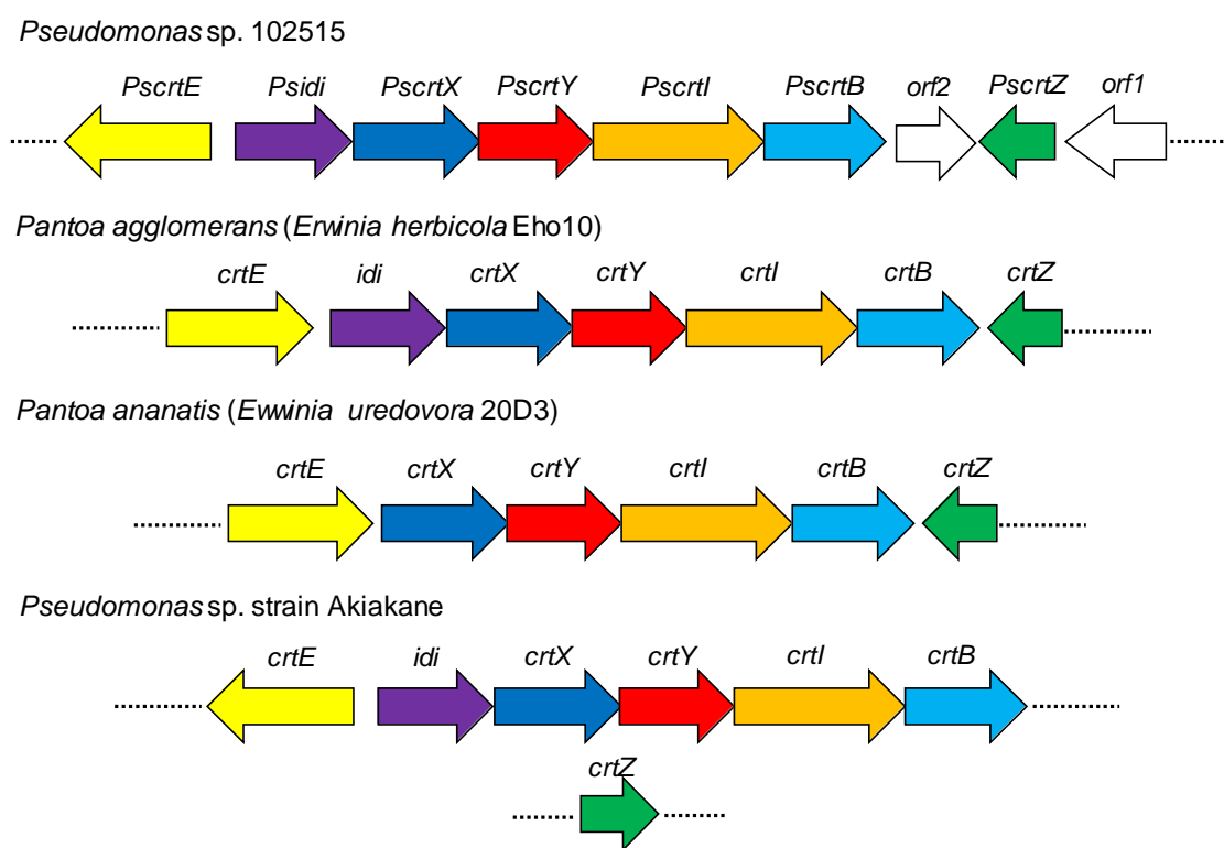
FIG. 19. Organization of carotenoid biosynthetic gene clusters in the \gamma -proteobacteria strains. NCBI accession numbers: M87280 for Pantoa agglomerans , CP001875 for Pantoa ananatis , and LC317091 and LC317092 for Pseudomonas sp. strain Akiakane.
