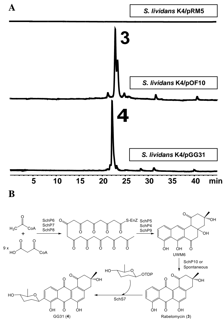
FIG. 4. Production of rabelomycin ( 3 ) and 9-D-amicetosyl-rabelomycin (GG31, 4 ) in S. lividans K4 through heterologous expression. (A) HPLC analysis (420 nm) of the products of S. lividans K4 harboring pRM5 (upper), pOF10 (middle) and pGG31 (bottom). (B) Biosynthetic pathway of 3 and 4 .
