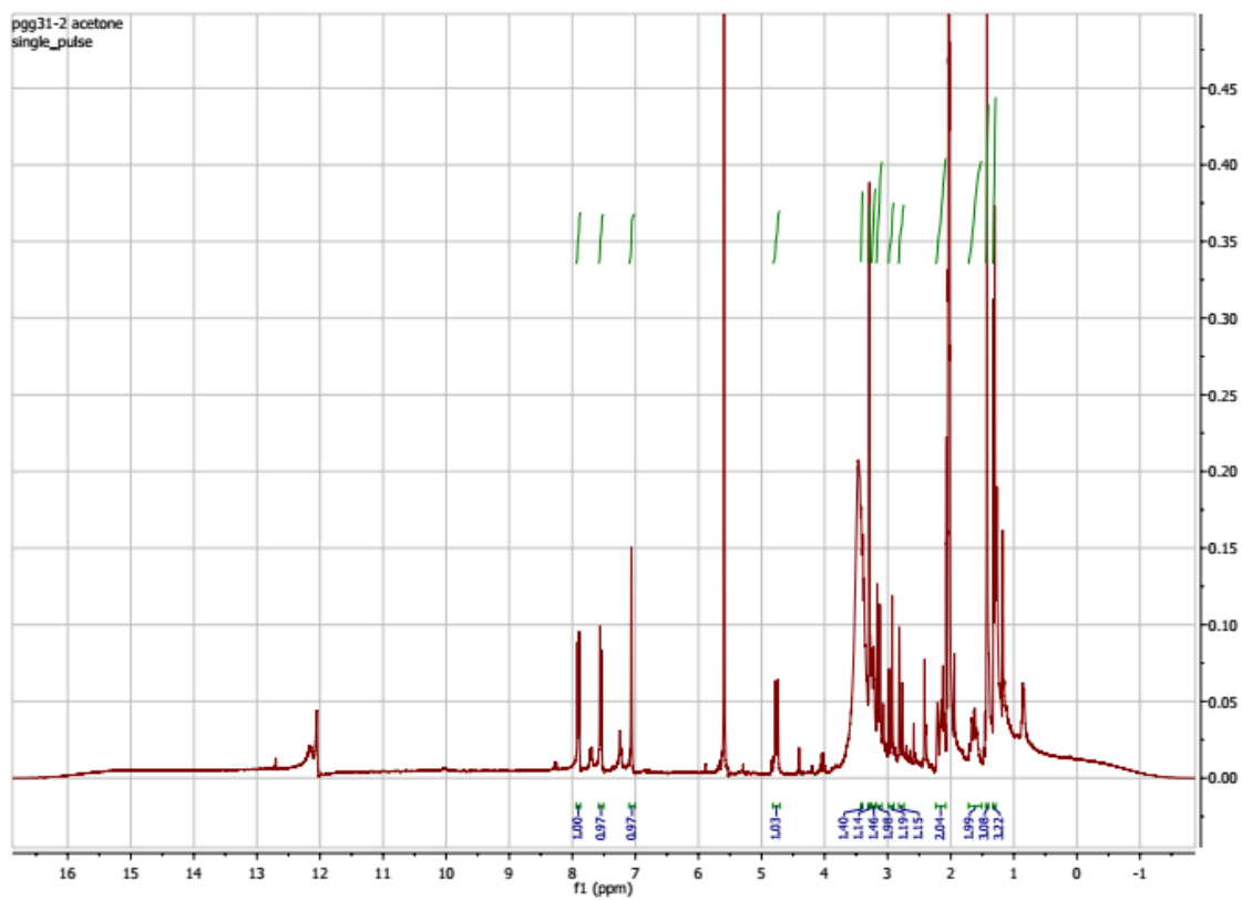
Fig. B3a. 1 H NMR for GG31 in (CD 3 ) 2 CO, 300 MHz, JEOL ECX-300.
