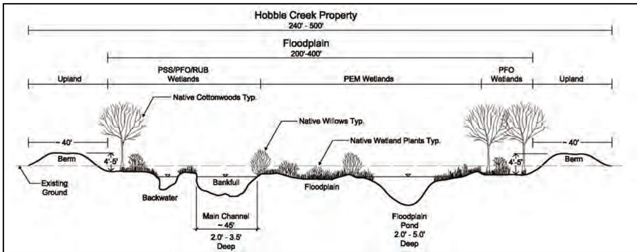
Figure 2.5. Cross section of Hubble Creek restoration design (DOI 2008).
