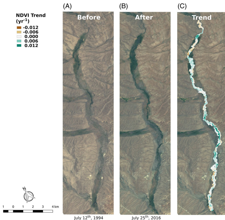
Figure 4. Aerial images of the Maggie Creek reach used in the evaluation from (A) before and (B) after restoration. (C) The linear trend in NDVI (calculated from Landsat satellite imagery) since restoration, representing increased vegetation productivity.
