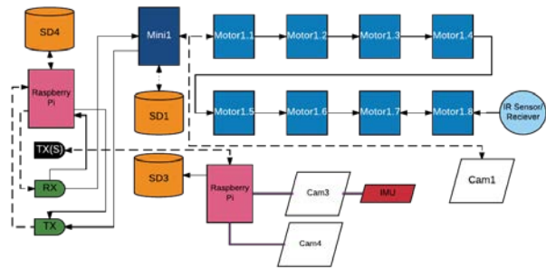
Figure 6: Software Layout
