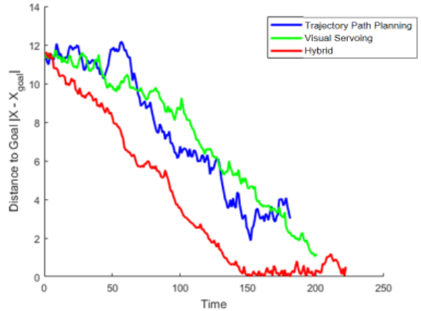
Figure 9: Simulation Results without Simulated Error
