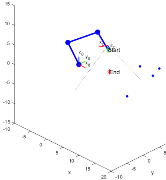
Figure 10: 3 DoF Simulation in 3D
