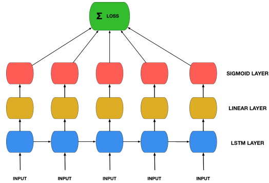
Figure 1: Our LSTM architecture
