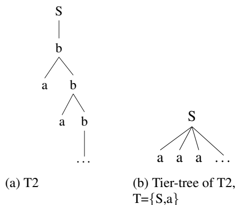
Figure 6: T2 and its tier-tree
