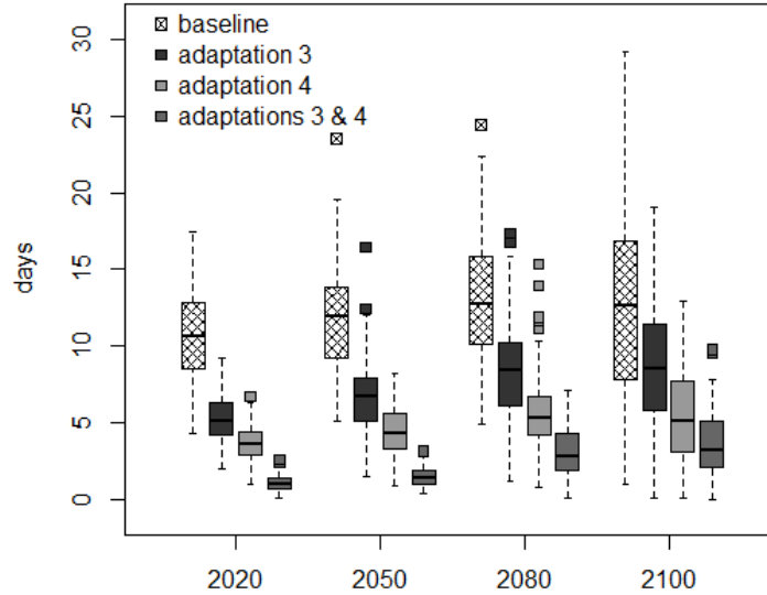
Figure 2.6 Average annual days of Alum addition in the Catskill Aqueduct for different climates and adaptations. The range of each boxplot shows the frequency of alum addition for each climate change scenario. For example, one outlier point represents one GCM output resulting in higher annual average alum use. The same set of climate scenarios are used for each decadal grouping of alternatives. The set of scenarios change in each decade to represent climate change over time. Four adaptation scenarios are shown in each decade.
