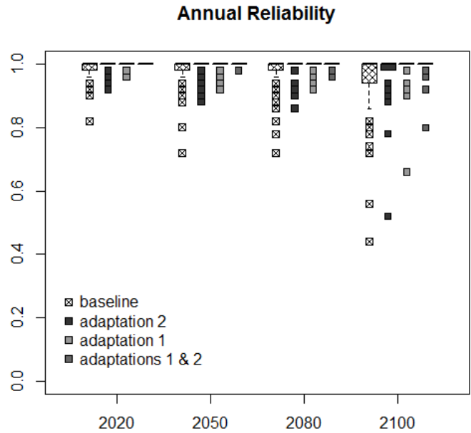
Figure 2.4 Annual reliability. The range of each boxplot shows system reliabilities in each climate change scenario. For example, one outlier point represents one GCM output resulting in lower annual reliability of the system. The set of scenarios change in each decade to represent climate change over time. Four adaptation scenarios are shown in each decade.
