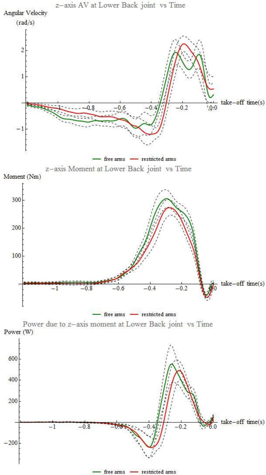
Figure 7: Angular velocity, moment and power about z-axis (pelvis anatomical reference frame) at lower back for the last 1.2 s before take-off for free and restricted arm jumps (mean \pm 95% CI)
