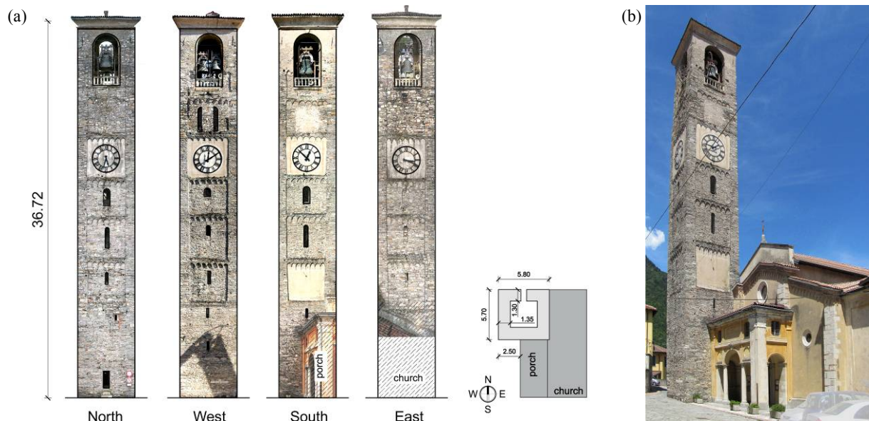
Figure 5: (a) Fronts and cross-section (dimensions in m) of the San Vittore bell-tower; (b) View of the bell-tower.
