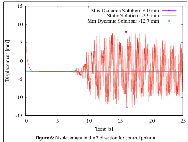
Figure 6: Displacement in the Z direction for control point A
