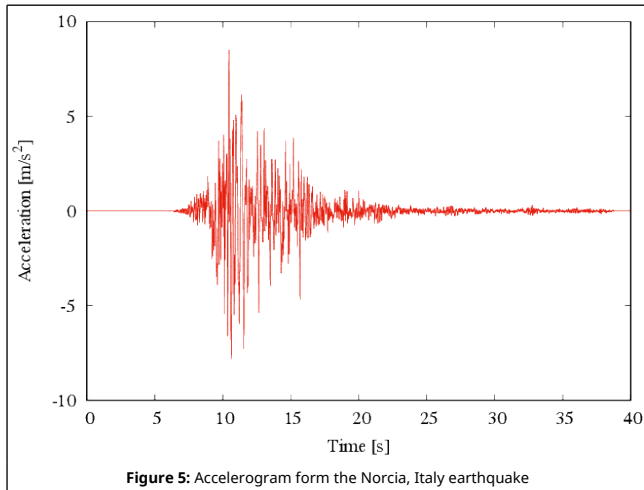
Figure 5: Accelerogram from the Norcia, Italy earthquake
