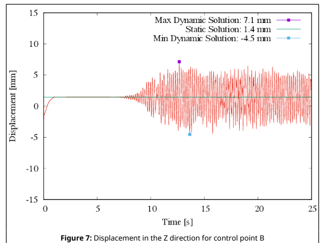
Figure 7: Displacement in the Z direction for control point B
