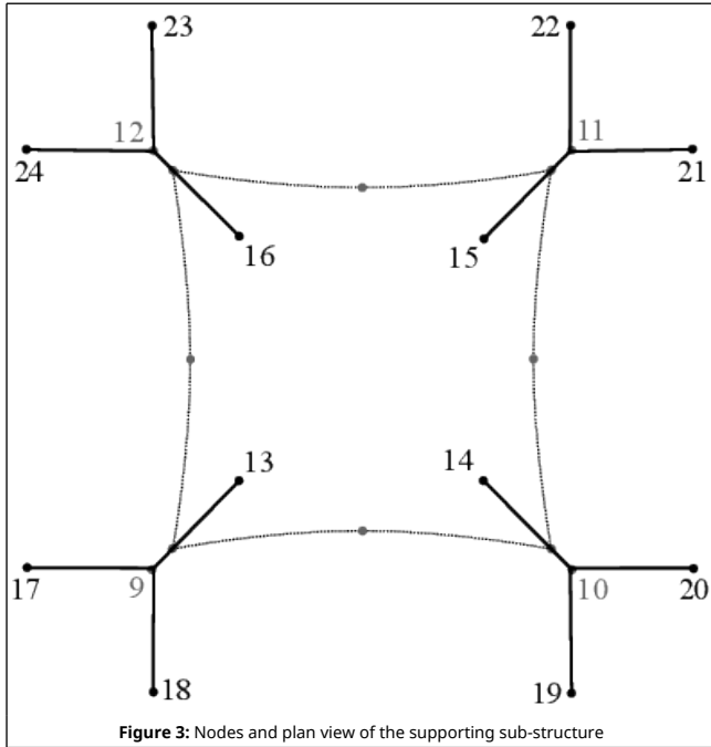
Figure 3: Nodes and plan view of the supporting sub-structure
