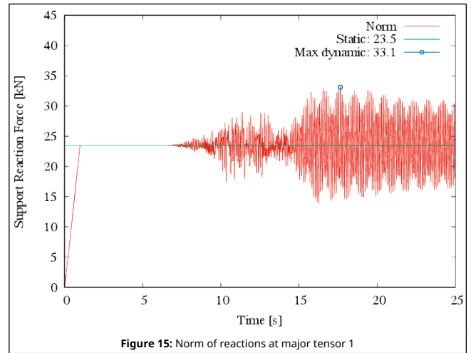
Figure 15: Norm of reactions at major tensor 1
