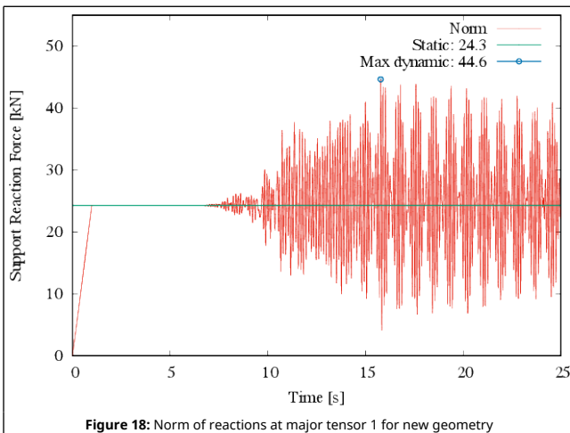
Figure 18: Norm of reactions at major tensor 1 for new geometry
