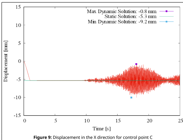
Figure 9: Displacement in the X direction for control point C
