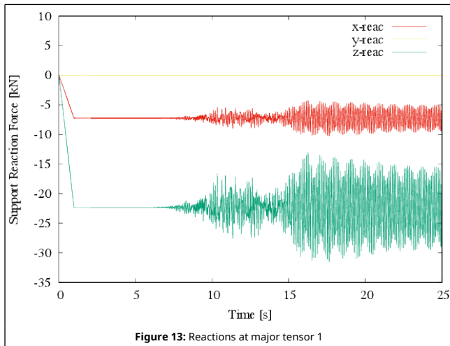
Figure 13: Reactions at major tensor 1
