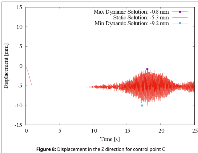
Figure 8: Displacement in the Z direction for control point C
