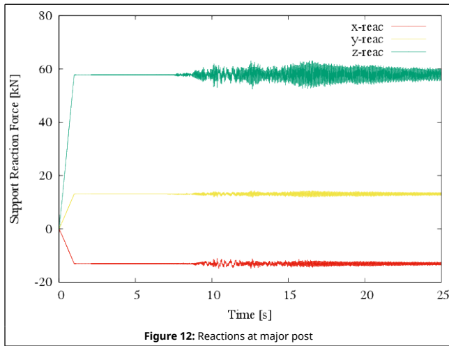
Figure 12: Reactions at major post
