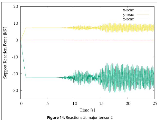
Figure 14: Reactions at major tensor 2
