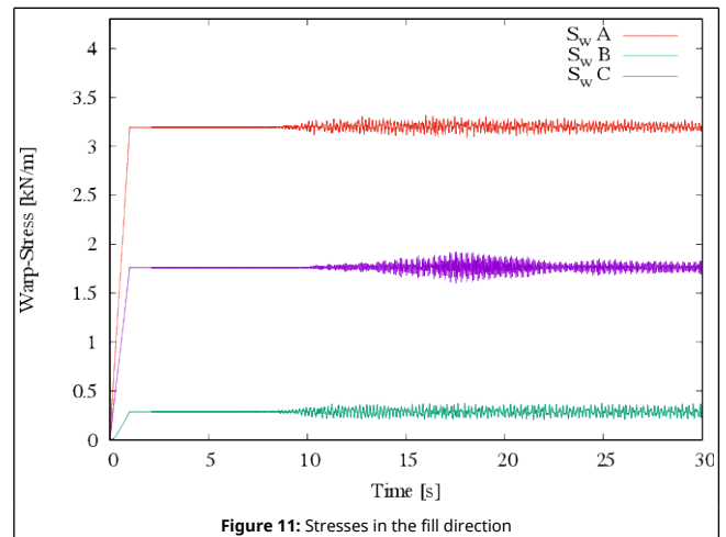
Figure 11: Stresses in the fill direction
