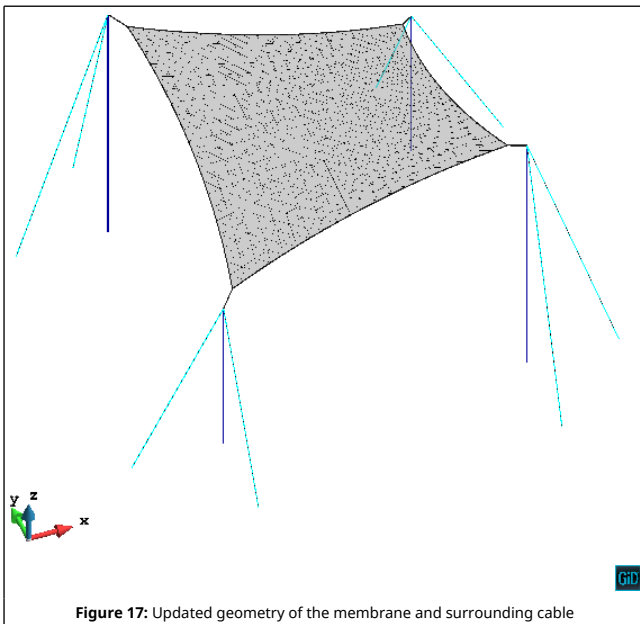
Figure 17: Updated geometry of the membrane and surrounding cable
