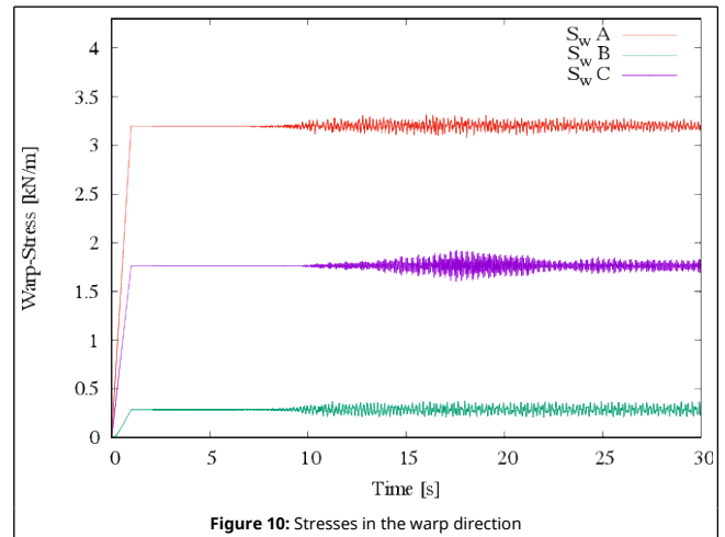
Figure 10: Stresses in the warp direction
