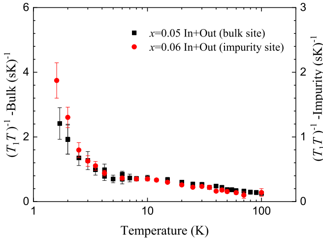
FIG. 13. Temperature dependence of the mean value of (T_1T)^{-1} of the associated inner and outer sites for bulk and impurity sites. The results of the bulk site are plotted with the left axis, and the results of the impurity site are plotted with the right axis.
