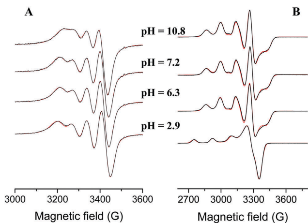
Fig. 5 Experimental (red) and simulated (black) EPR spectra of the copper(II)–L 1/1 system at room temperature (A) and at 77 K (B). ([L] = [\text{Cu}^{2+}] = 2.96 mM, I = 0.1 M (NaCl)).
