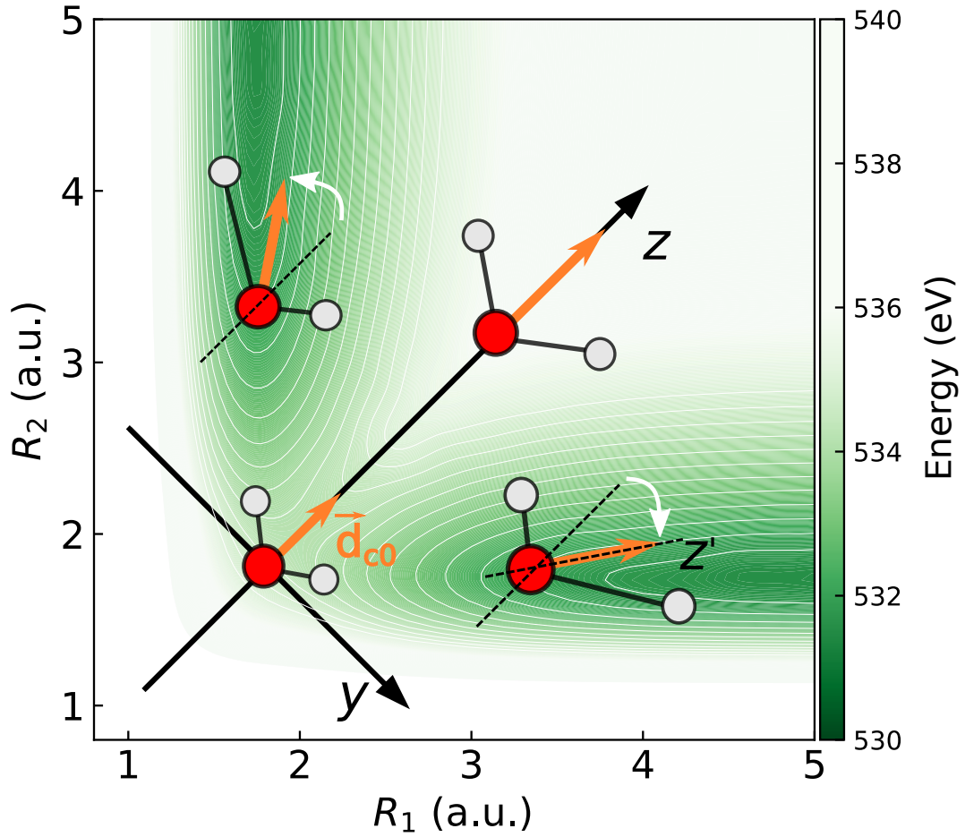
FIG. 2. Schematic picture of opposite rotation of the transition dipole moment in the course of coherent dissociation along different pathways. The green colormap displays the potential energy surface of the dissociative |O1s^{-1}4a_1^1\rangle core-excited state as function of the bond lengths R_1 and R_2 . The transition dipole moment \mathbf{d}_{c0} is shown by the orange arrows.
