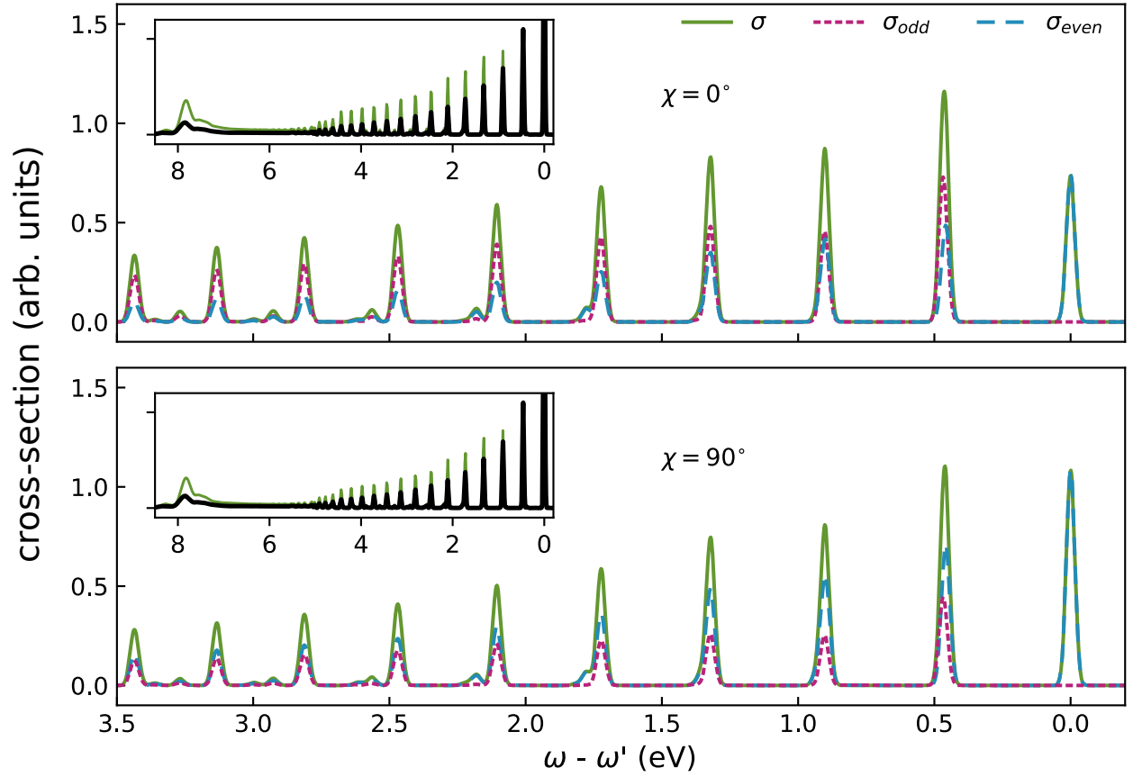
FIG. 5. Total cross-section \sigma (solid green) and partial cross-sections \sigma_{odd} (dotted red) and \sigma_{even} (dashed blue) (Eq. 17) for \chi = 0^\circ (upper panel) and \chi = 90^\circ (lower panel). The inserts in both panels compare the strict \sigma (thin green) and \sigma computed using the FC approximation (thick black). The spectra are normalized so that the peak n = 1 in \sigma equals 1.
