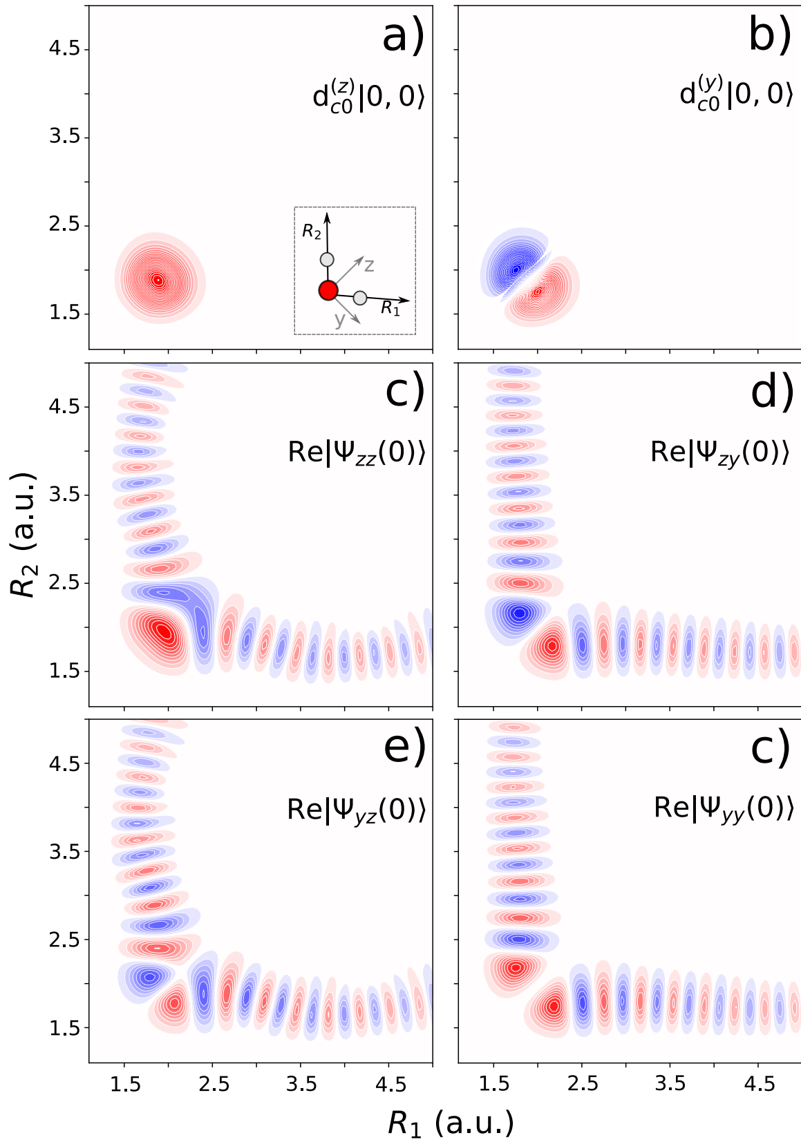
FIG. 4. Panels a) and b) show how the z - and y -components of the transition dipole moment effectively change the symmetry of the initial vibrational state. Panels c)-f) show that contrary to \Psi_{zz}(0) and \Psi_{yy}(0) the y -component of \mathbf{d}_{c0} makes antisymmetric the wave packets \Psi_{zy}(0) and \Psi_{yz}(0) .
