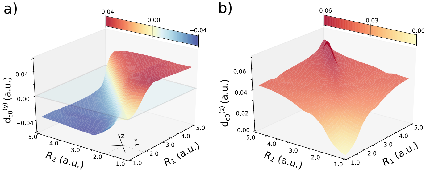
FIG. 1. Surfaces of the components of the transition dipole moment \mathbf{d}_{c0} as functions of the bond lengths R_1 and R_2 . Panel a) displays the anti-symmetric y component while panel b) shows the symmetric z component.
