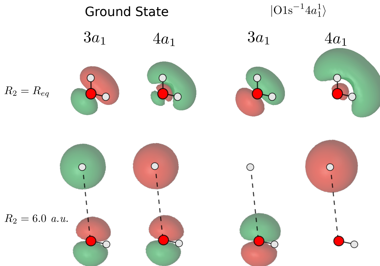
FIG. 3. Natural orbitals involved in the dissociation of the OH bond. The orbitals are extracted from the multi-electronic RASSCF wavefunctions of the ground state and the |O1s^{-1}4a_1^1\rangle core-excited state. The upper row displays the 3a_1 and 4a_1 orbitals at equilibrium geometry R_1 = R_2 = R_{eq} = 1.81 \text{ a.u.} while the bottom row shows the same in the region of dissociation R_1 = R_{eq} = 1.81 \text{ a.u.} , R_2 = 6 \text{ a.u.}
