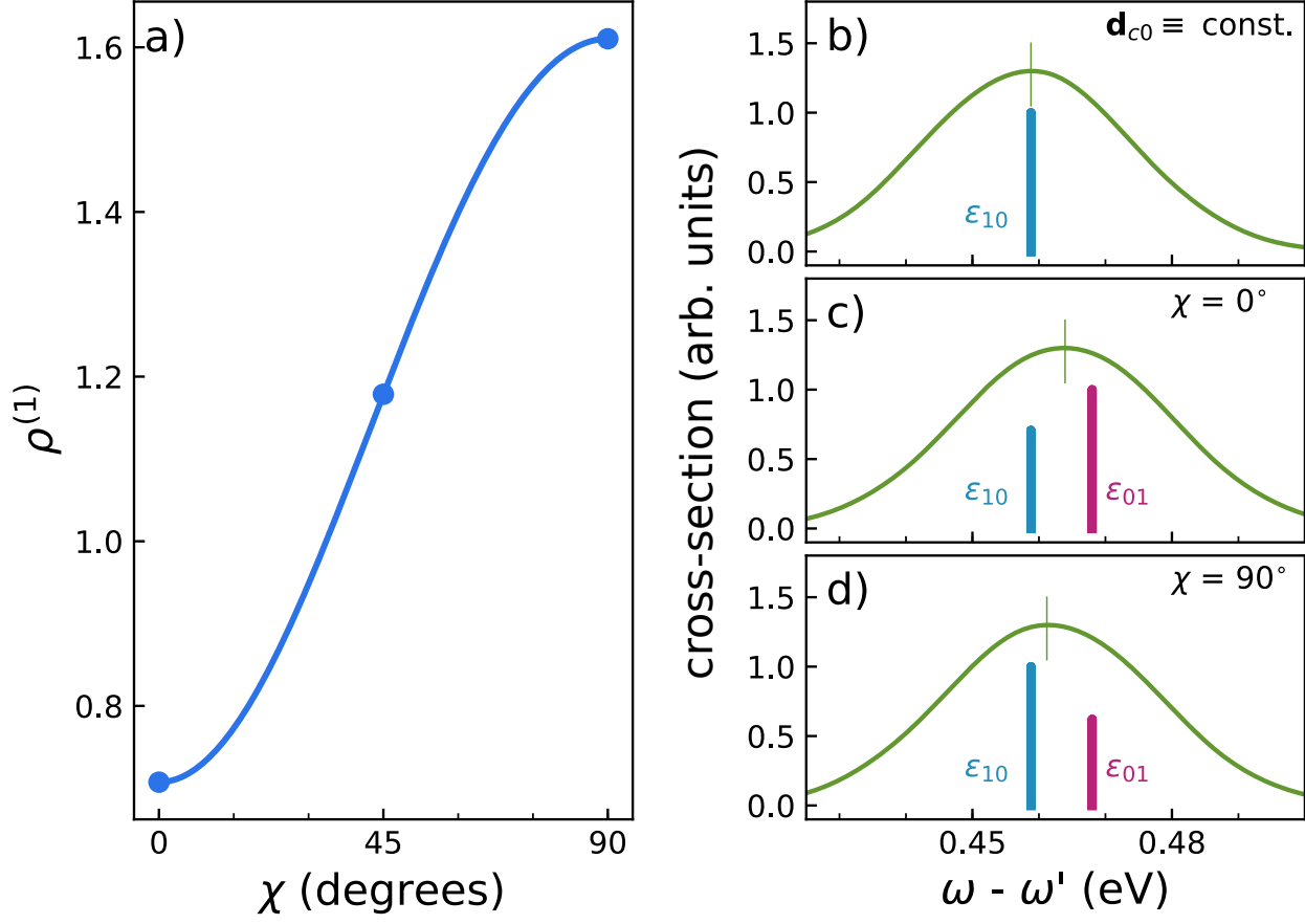
FIG. 7. a) Polarization dependence of the ratio \rho^{(1)} of intensities of the symmetry allowed (10) and forbidden (01) RIXS channels (see eq.(19)). Panel b) displays \sigma for the peak n = 1 in the FC approximation. Panels c) and d) show the same taking into account the rotation of the transition dipole moment for \chi = 0^\circ and 90^\circ , respectively. The total profile shown by thick green line is calculated using a Gaussian with half-width at half maximum equal to 0.02 eV. The RIXS cross-section bars for levels \epsilon_{1,0} and \epsilon_{0,1} are shown by thick blue and magenta bars, respectively. The vertical thin green lines show weak dependence of the peak position of unresolved peaks on the scattering angle \chi .
