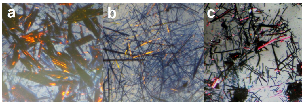
Figure 2. Microscopic images of PdPc (a), PdPcF 4 (b) and PdPcF 16 (c) crystals suspended in liquid epoxy.
