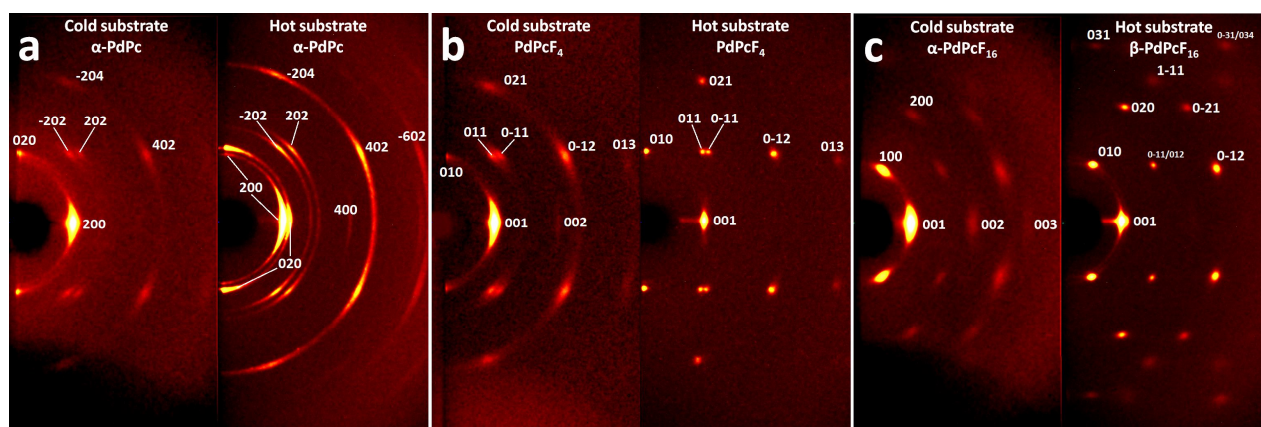
Figure 5. 2D GIXD patterns for the film of PdPc (a), PdPcF 4 (b) and PdPcF 16 (c), deposited on cold (left image) and hot (right image) substrates.
