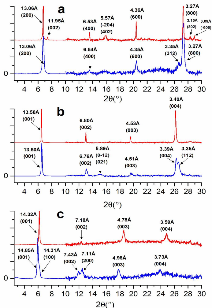
Figure 4. X-ray diffraction patterns of thin films of PdPc (a), PdPcF 4 (b) and PdPcF 16 (c), deposited on cold (blue lines) and hot (red lines) substrates.
