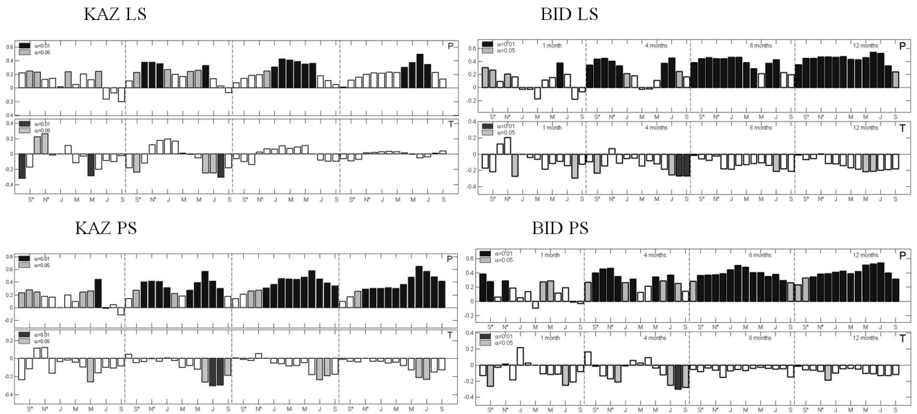
Fig. 5. Climatic response of tree-ring chronologies calculated in the Seascorr program for seasons of 1, 4, 8, and 12 months. The primary limiting factor is precipitation, and the secondary limiting factor is temperature. Last month of period is labeled on the horizontal axis
