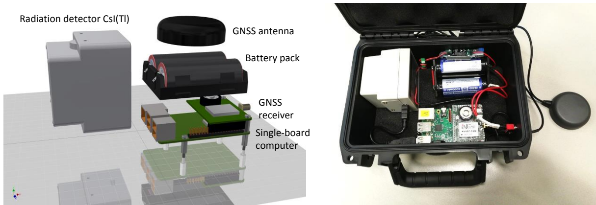
Figure 1. Components of the IEC 63047 demonstration device.
