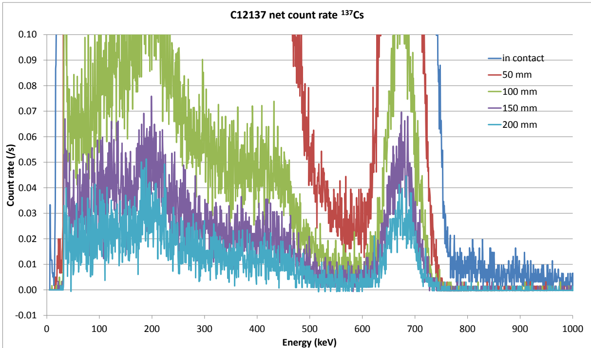
Figure 9. Net count rate spectrum showing pile-up of events when the source is in contact with the small detector.
