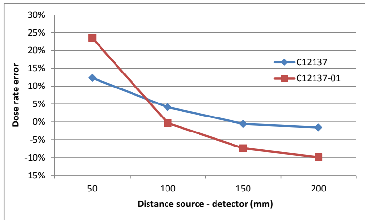
Figure 7. Error on the dose rate.
