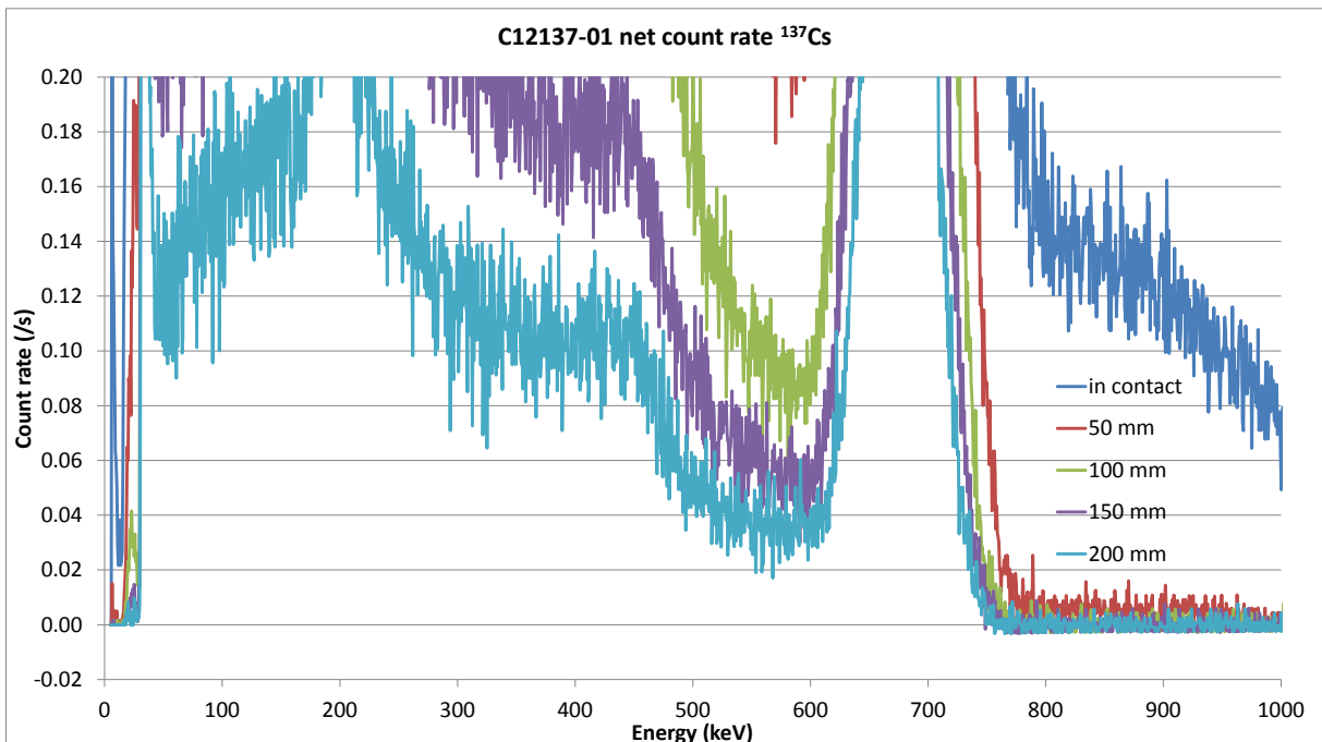
Figure 10. Net count rate spectrum showing pile-up of events when the source is in contact with the larger detector. The pile-up effect is also present when the source is at a distance of 50 mm.
