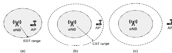
Fig. 1: An illustration of possible Wi-Fi AP positions with respect to LTE-U eNB, depicting the three scenarios: (a) Inside EDT range, (b) In-between EDT and CST range, (c) Outside CST range.
