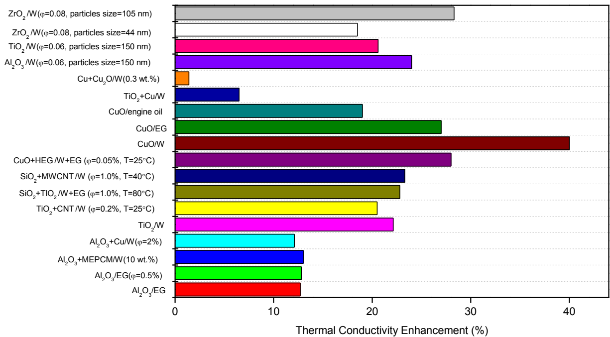
Figure 1. The variation of thermal conductivity enhancement for different type of metal oxide nanofluids.
