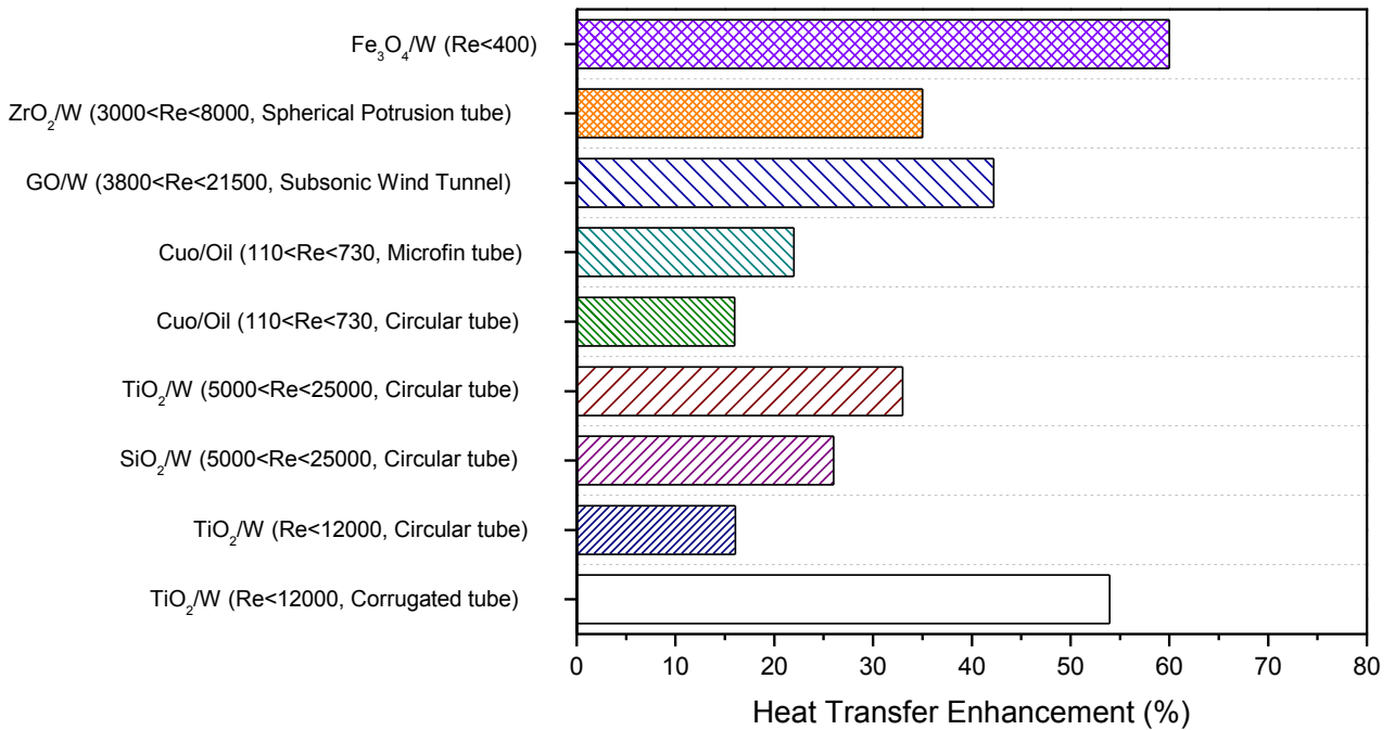
Figure 2. The variation of heat transfer augmentation for various types of metal oxide nanofluids in a plain tube.
