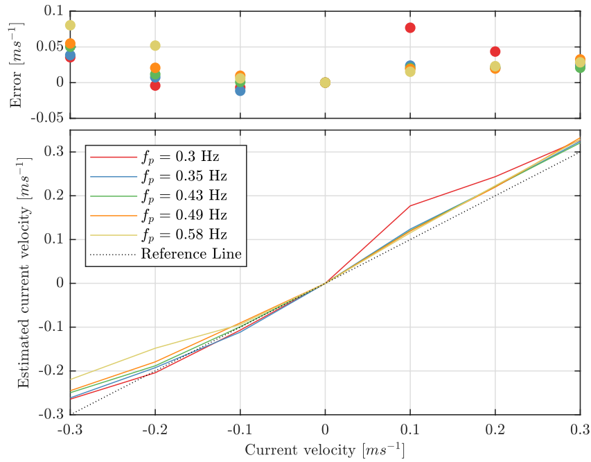
Fig. 12. Error and correlation in estimated current velocities for 5 p.m. spectra of differing peak frequency. The data are calculated for spectra created in currents ranging from -0.3\text{m/s} . to 0.3\text{m/s} R^2 = 0.99 and \text{RMSE} = 0.031\text{ m s}^{-1} .
