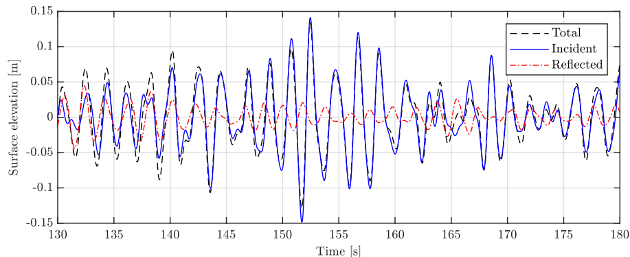
Fig. 11. Example of time-series reconstruction of incident, reflected and total surface elevations. Shown for f_p = 0.4922 Hz, 0.20\text{m s}^{-1} current following waves at x = 0
