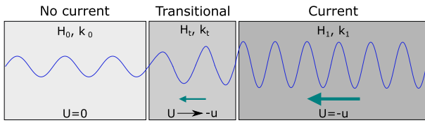
Fig. 1. Diagram showing wave propagating from region of no current to a region with current. Change in wave height and wavelength (wavenumber) due to interaction with current field indicated. Example shown with opposing current (negative u ) where wave height increases and wavelength decreases (Draycott et al., 2018).
