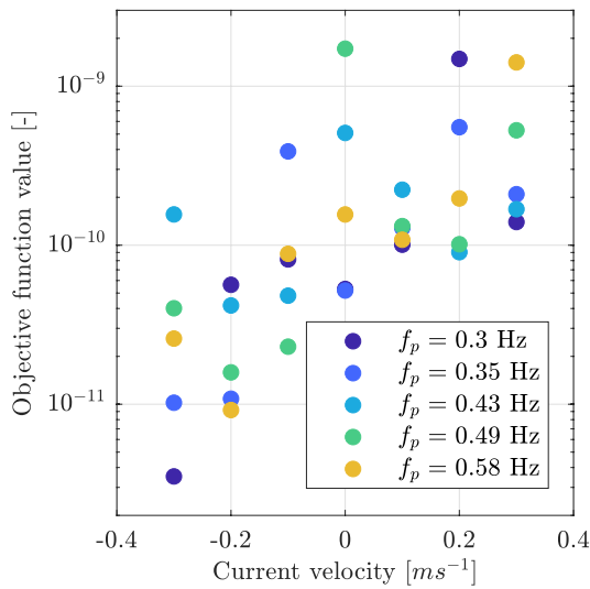
Fig. 6. Converged objective function values for each of the 35 experiments.
