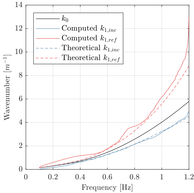
Fig. 10. Wave numbers for current following waves, f_p = 0.4922 Hz, 0.20\text{m s}^{-1} current following waves.
