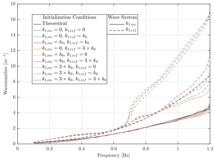
Fig. 13. Sensitivity to initialization of wavenumbers in IPOPT for current following waves, f_p = 0.4922\text{ Hz} , 0.20\text{m s}^{-1} current following waves.
