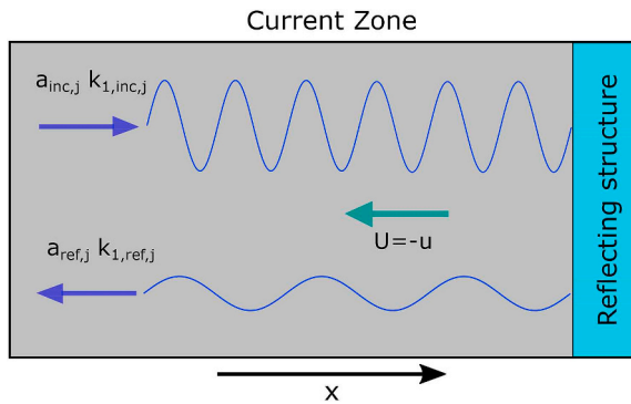
Fig. 2. The wave field in the measurement (current) zone is made up of incident and reflected components from a structure. In the diagram the reflecting structure is shown inside the current zone but could equally be outside. Highlights that for a given frequency component, j , that there exist two wavenumbers and amplitudes for each frequency. Shown here with opposing current (negative U ) where wavelength decreases for incident, and increases for reflected wave components (Draycott et al., 2018).
