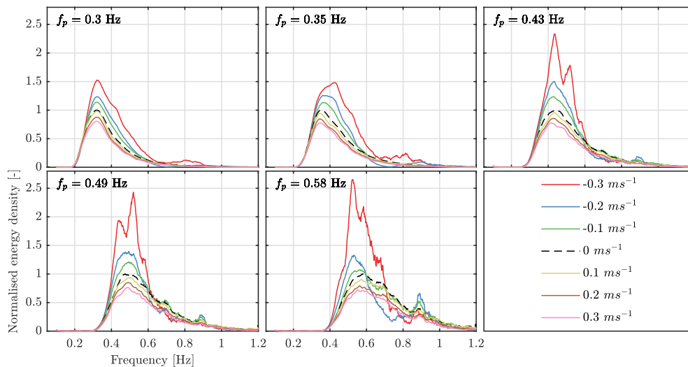
Fig. 7. Incident frequency spectra for 5 p.m. spectra of differing peak frequency. The data are calculated for spectra created in currents ranging from -0.3\text{m s}^{-1} to 0.3\text{m s}^{-1} .
