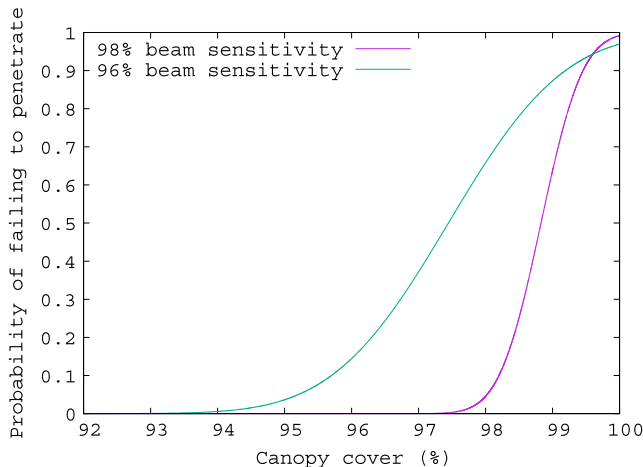
Figure 3. Probability of waveforms to detect the ground against canopy cover for two different beam sensitivities.
