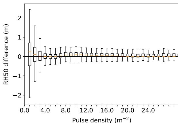
Figure 10. Boxplots of difference between RH50 derived from simulated Land, Vegetation, and Ice Sensor waveforms from airborne laser scanning data sets with different survey configurations over the same site, using the highest laser pulse rate (RIEGL Q680), lowest altitude data set as the baseline.
