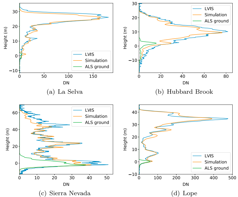
Figure 4. Comparison of four individual simulated and observed LVIS waveforms with the ground portion of the simulated waveform shown. LVIS = Land, Vegetation, and Ice Sensor; ALS = airborne laser scanning; DN = digital number. Examples are shown for La Selva (a), Hubbard Brook (b), Sierra Nevada (c), and Lope (d).
