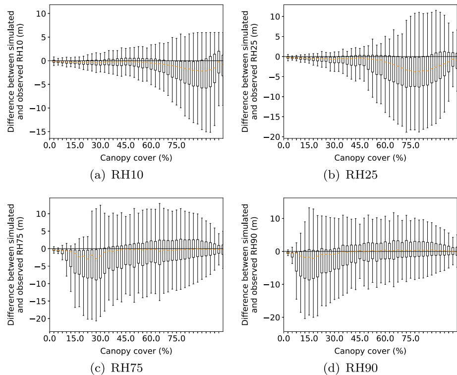
Figure 7. Difference between simulated and observed Land, Vegetation, and Ice Sensor RH metrics against canopy cover over Mabounie, showing a ripple of uncertainty at a canopy cover equal to one minus that RH metric. RH = relative height. Examples are shown for RH10 (a), RH25 (b), RH75 (c), and RH90 (d).
