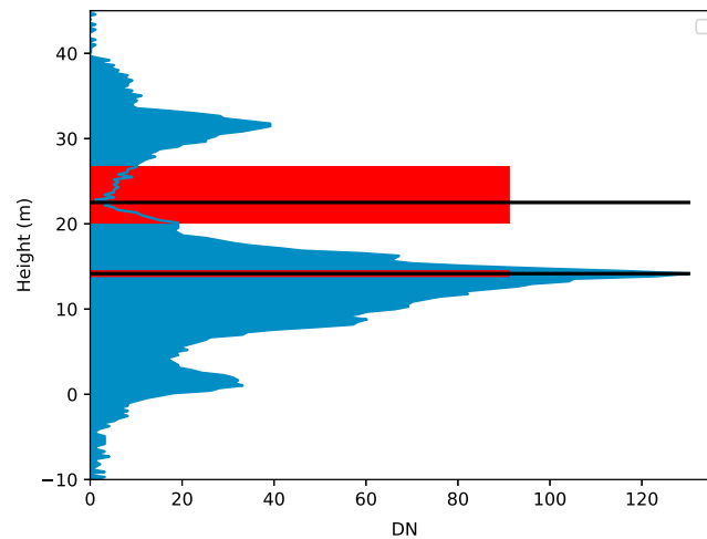
Figure 8. Illustration of distance a 2% change in energy can cause for relative height metrics at points of high and low waveform intensity. Black lines mark RH50 and RH80. Red boxes indicate a shift that would result with a \pm 2\% energy change.
