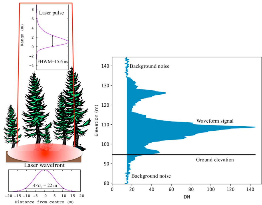
Figure 1. Illustration of Global Ecosystem Dynamics Investigation instrument characteristics and how they contribute to the measured waveform shape.
