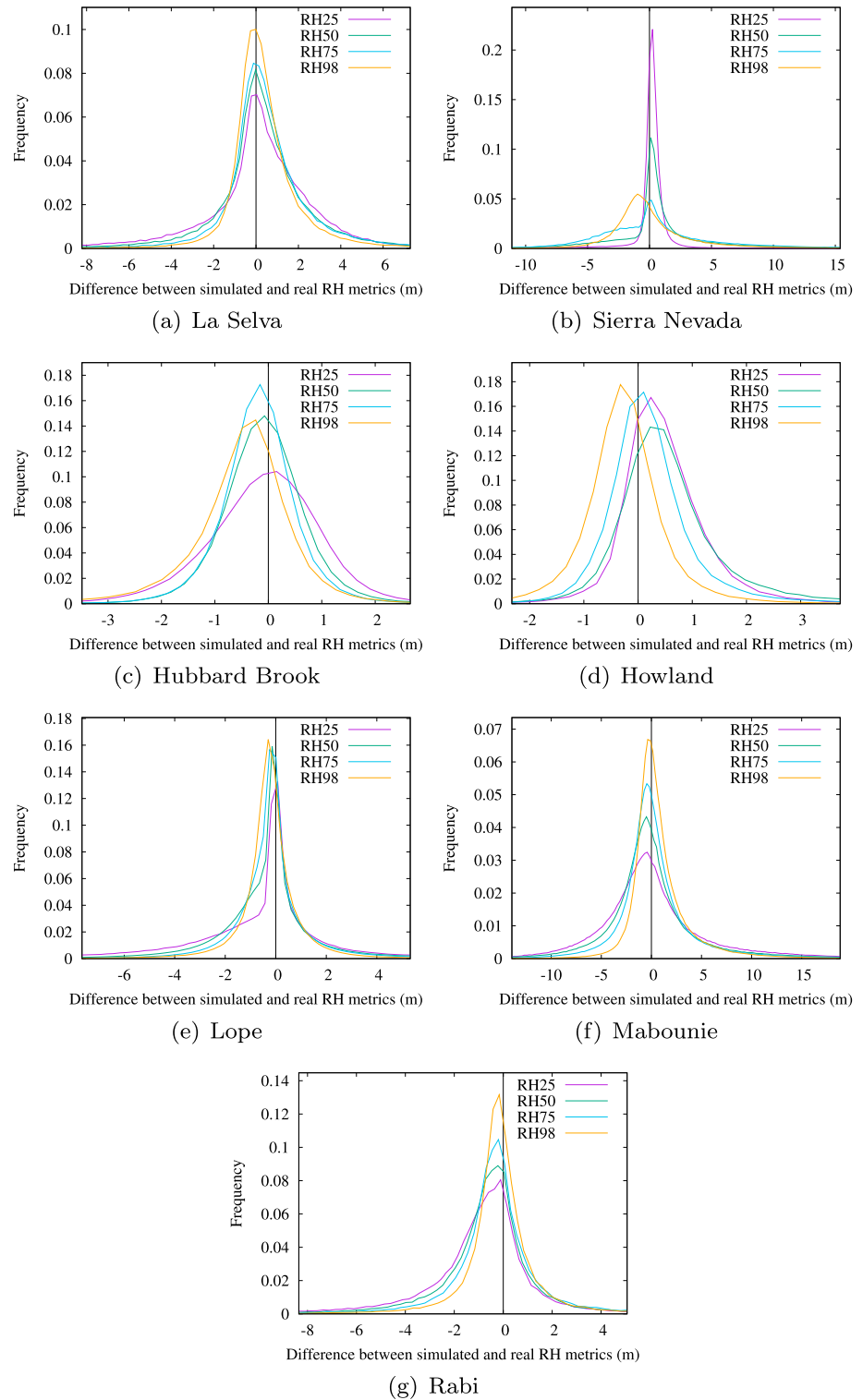
Figure 9. Histograms of difference between observed and simulated Land, Vegetation, and Ice Sensor RH metrics for the count method with airborne laser scanning pulse density normalization. Examples are shown for La Selva (a), Sierra Nevada (b), Hubbard Brook (c), Howland (d), Lope (e), Mabounie (f), and Rabi (g) RH = relative height.
