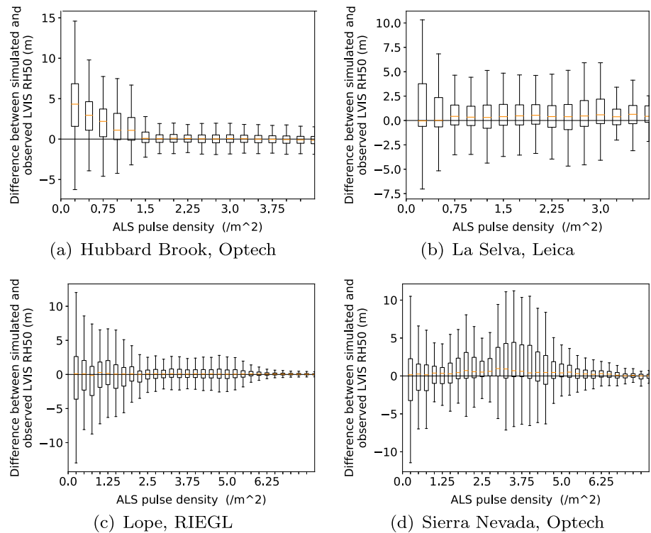
Figure 5. Boxplots showing the difference between RH50 from simulated and observed LVIS waveforms against ALS pulse density for Hubbard Brook (a), La Selva (b), Lope (c) and Sierra Nevada (d). The boxes show the interquartile range (25th and 75th percentile), the bar the median and the whiskers are 1.5 times the interquartile range long. Outliers have been excluded from this plot and will be investigated in detail later, along with the higher root-mean-square error at Sierra Nevada around 3.5 pulses per square meter.
