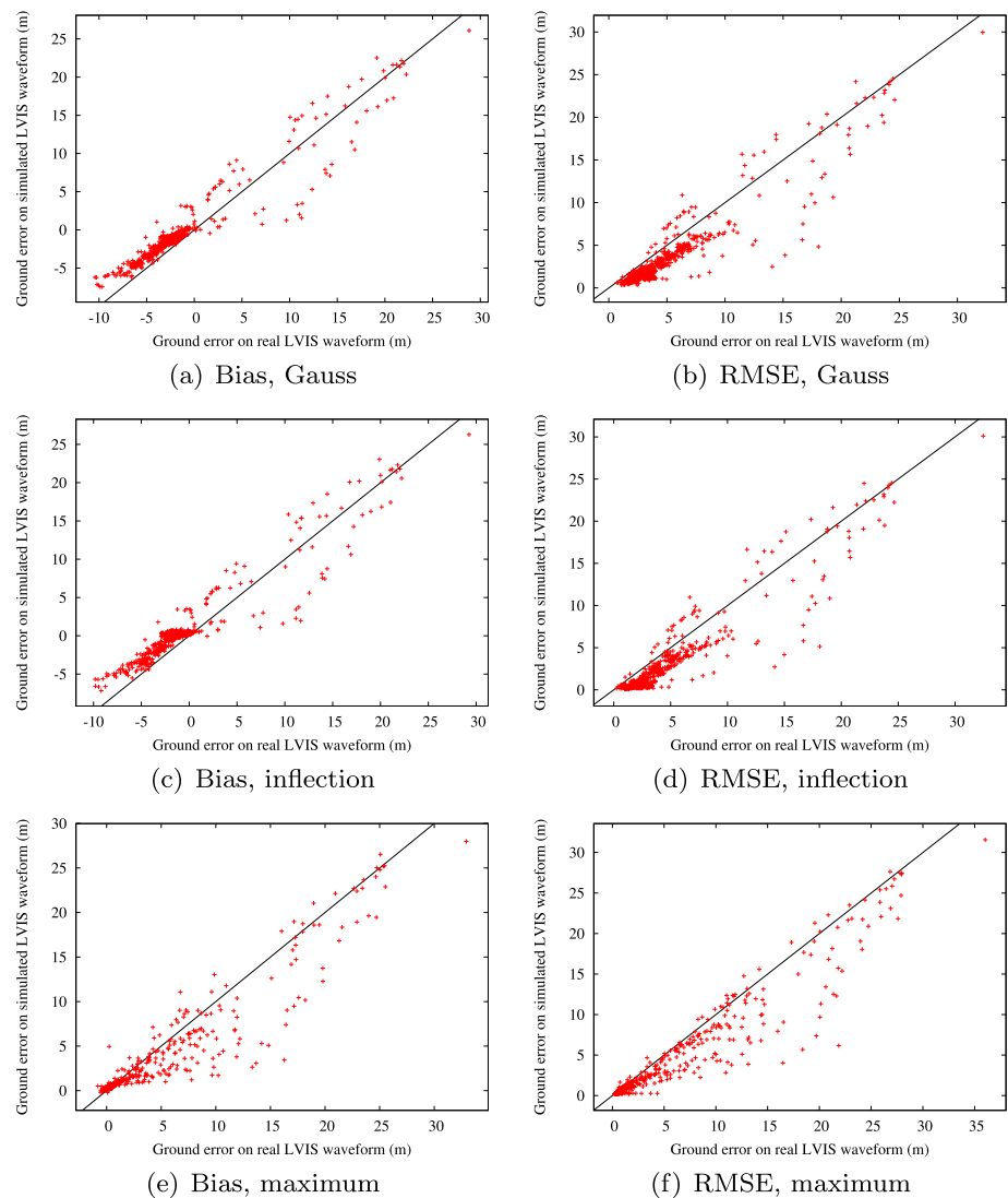
Figure 12. Scatterplots of ground-finding error on observed and simulated noisy LVIS data, binned by canopy cover, slope, and beam sensitivity across all sites for three ground-finding algorithms; Gauss (bias (a), RMSE (b)), inflection (bias (c), RMSE (d)), and maximum (bias (e), RMSE (f)). LVIS = Land, Vegetation, and Ice Sensor; RMSE = root-mean-square error.
