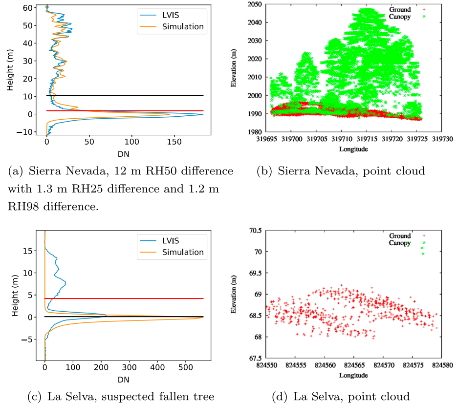
Figure 6. Examples of simulated and observed LVIS waveforms with large RH50 differences. Examples are shown for Sierra Nevada (waveforms (a) and point cloud (b)) and La Selva (waveforms (c) and point cloud (d)). LVIS = Land, Vegetation, and Ice Sensor; DN = digital number.
