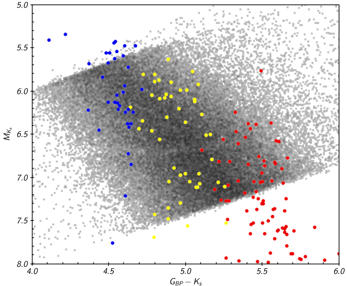
Figure 6. An observational HRD using G_{BP} - K_s and M_{K_s} to separate different spectral types of stars. Blue, yellow and red circles represent known single stars within 25 pc with spectral types of M2.0V, M3.0V, and M4.0V, respectively.
