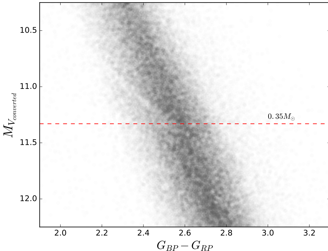
Figure 9. An observational HRD using G_{BP} - G_{RP} and M_{V_{converted}} is shown. The red dashed line that intersects the gap marks the M_{V_s} = 11.33 value that corresponds to stars with mass 0.35M_{\odot} based on the mass-luminosity relation of Benedict et al. (2016) from nearby stars with various metallicities.
