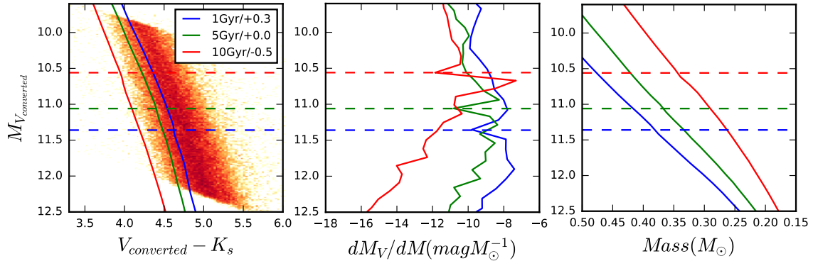
Figure 8. Three different isochrones (solid lines) from YaPSI are plotted against the Gaia data on the HRD. Blue, green and red lines represent three different isochrones, 1Gyr/[Fe/H]=+0.3/X=0.717/Z=0.03, 5Gyr/[Fe/H]=+0.0/X=0.733/Z=0.016 and 10Gyr/[Fe/H]=-0.5/X=0.744/Z=0.005, respectively, and all isochrones have Y=0.25 . The Gaia BP magnitudes are converted to V using the relation discussed in Appendix A. We note that these isochrones do not contain 2MASS K_s magnitudes, but we believe the difference between K and K_s is small. The middle plot is the slope of the mass-luminosity relations of these three metallicities shown on the right. Three colored dashed lines mark where the MLR slopes have local minima at M_V = 11.36 , 11.06 and 10.56.
