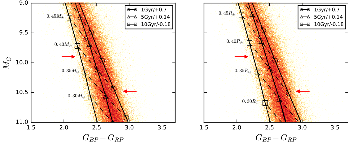
Figure 7. Three different isochrones (solid lines) from PARSEC are shown on the HRD. Circles, triangles and square boxes represent three different isochrones given in the legends. Dashed lines represent equal masses (left figure) and radii (right figure) on all three isochrones. Because these two figures are crowded, identifying this gap becomes difficult. Two arrows mark the gap location and the gap feature appears to have a shallower slope than either the equal-mass line at 0.4M_{\odot} or equal-radius line at 0.4R_{\odot} .
