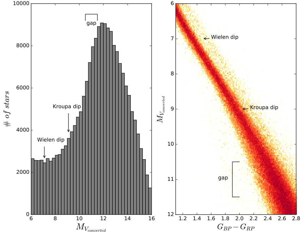
Figure 5. (Left) The stellar luminosity function based on Gaia DR2 data is shown. The Johnson V magnitudes have been converted using the transformation discussed in Appendix A. The “Wielen dip” and “Kroupa dip” are roughly marked at M_V \approx 7 and 9 , respectively. The gap discussed here is outlined with a bracket shown at M_V=10.5-11.5 . (Right) The different dips and the DR2 gap are marked on the HRD, and this DR2 gap is very obvious.
