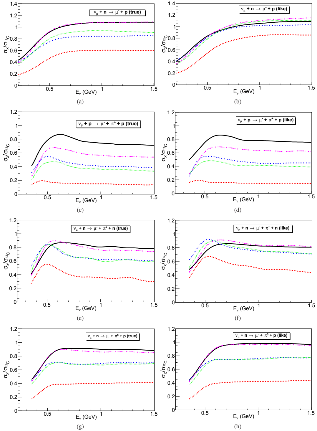
FIG. 4. (Color online) Inclusive muon neutrino-nucleus cross section ratios relative to ^{12}\text{C} , \mathcal{R} = \sigma_X/\sigma_{12\text{C}} , for different channels as function of neutrino energy: (solid black line) ^{16}\text{O} , (dash dot dot dot rouge line) ^{27}\text{Al} , (dot green line) ^{56}\text{Fe} , (dash dot blue line) ^{40}\text{Ar} , (dot red line) ^{208}\text{Pb} . Left panel: true-type and Right panel: like-type events.
