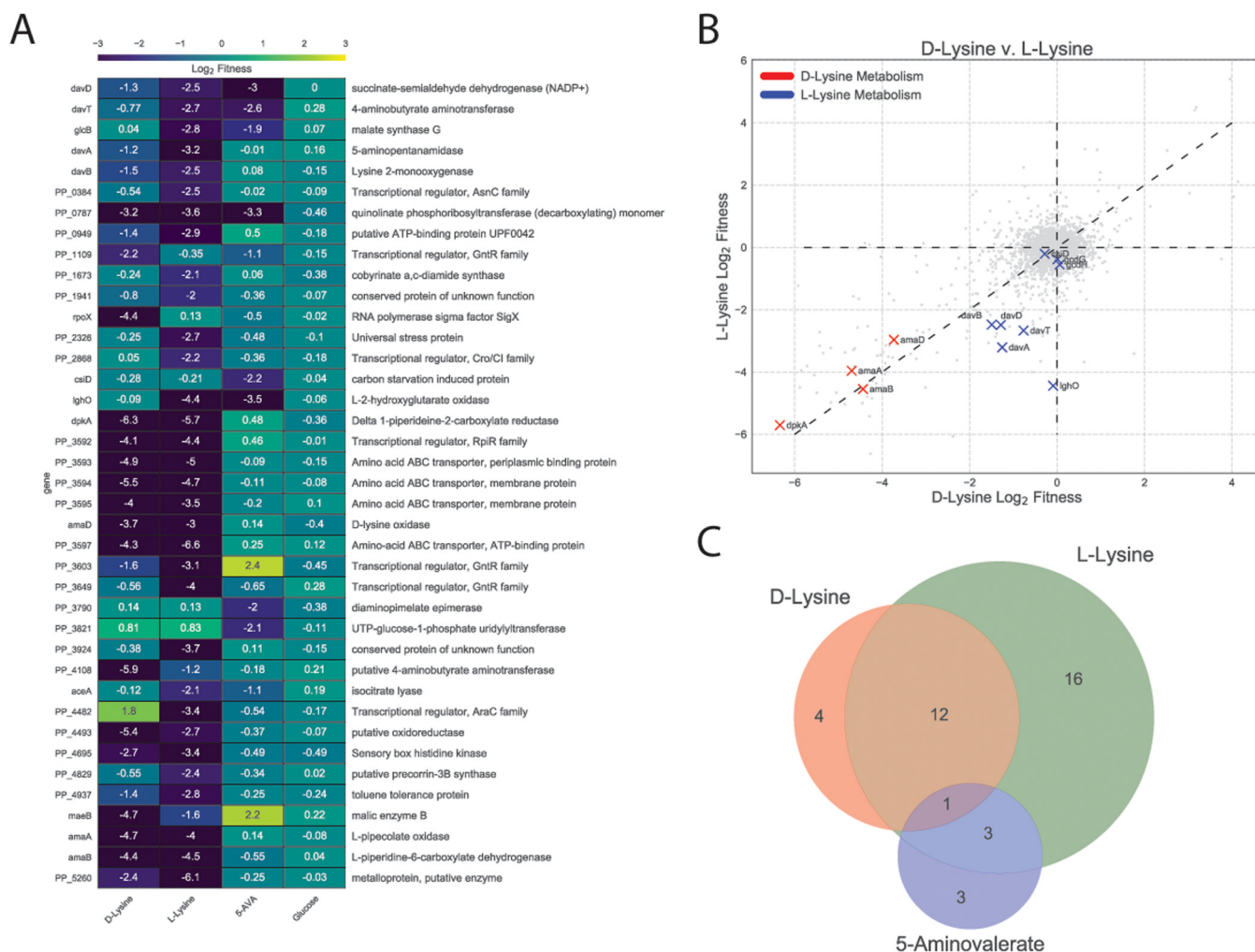
FIG 1 Results of RB-TnSeq screen. (A) Genes that showed less than -2 \log_2 fitness on D-lysine, L-lysine, or 5AVA but showed a fitness defect of no less than -0.5 \log_2 when grown on glucose. (B) Plot of genome-wide fitness values of libraries grown on either L-lysine or D-lysine. Genes encoding enzymes known to be involved in D-lysine metabolism are shown in red, while those known to be involved in L-lysine metabolism are shown in blue. (C) Venn diagram of genes with significant fitness defects when grown on D-lysine, L-lysine, or 5AVA.
