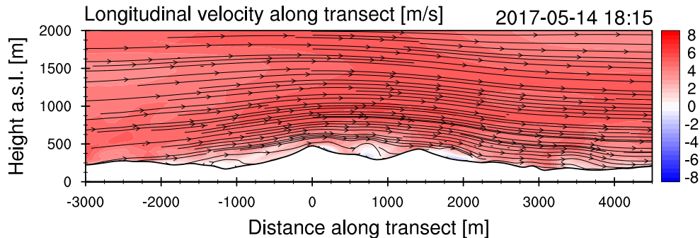
Figure 3: 14 May 2017 18:15 UTC. Streamlines and longitudinal velocity. Computational results are VENTOS ® /M micro-scale results (40 m grid) coupled with WRF results (1.5 km grid), based on input data from NCEP; the terrain is plotted in white.
