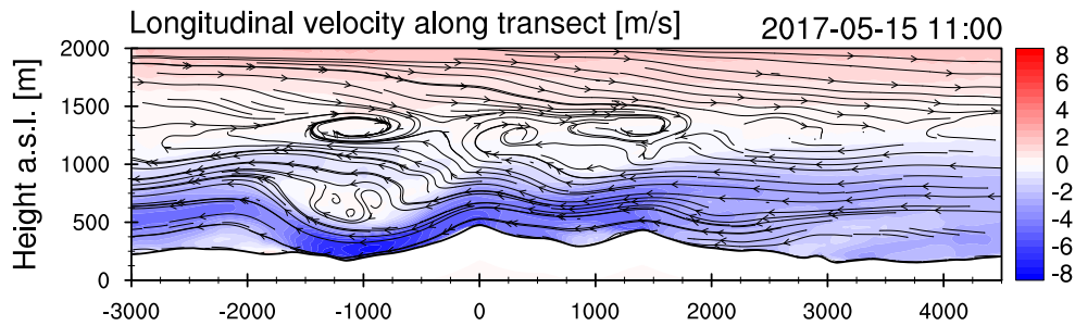
(a) Streamlines and longitudinal velocity. Computations as in Figure 3.
