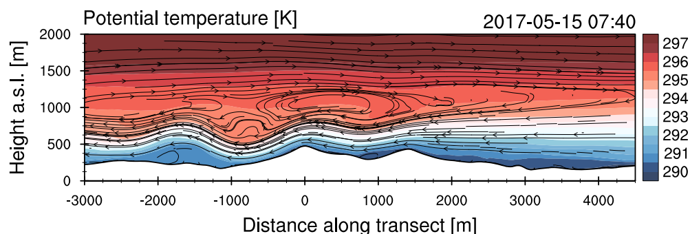
(c) Potential temperature. Computations as in Figure 3.
