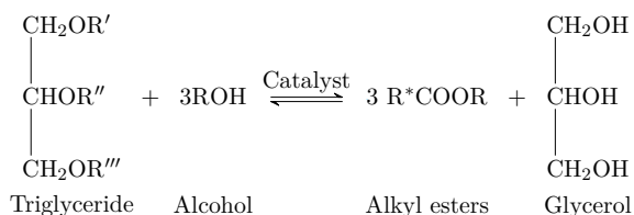
Figure 3.1: Transesterification of triglyceride with alcohol.
