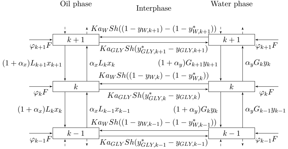
Figure 5.6: Schematic diagram of the finite volume model for the counter-current spray column.
