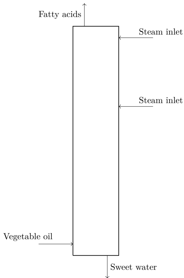
Figure 5.4: Counter-current spray column.
