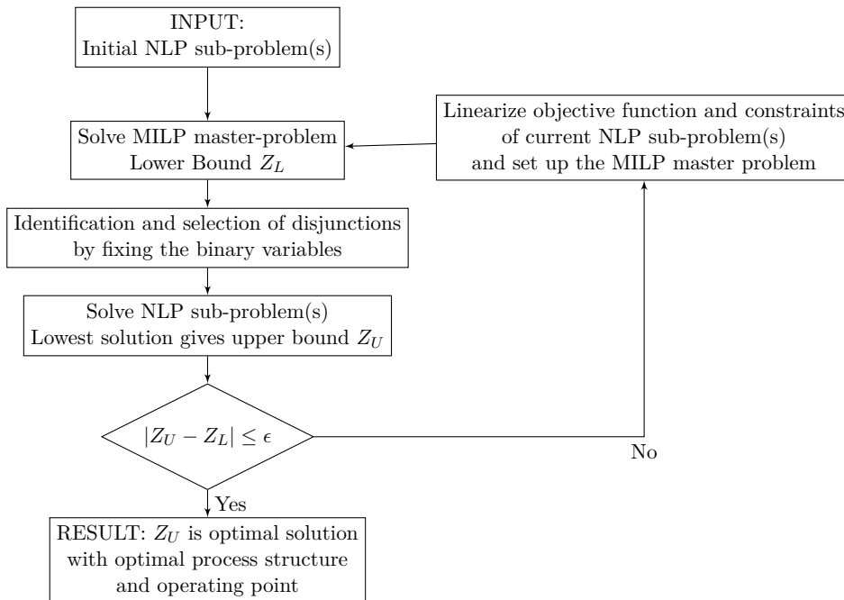
Figure 6.4: Logic-based outer approximation flow diagram.
