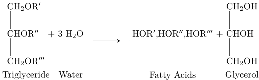
Figure 5.2: Hydrolysis reaction of triglycerides with water to give fatty acids and glycerol.
