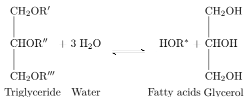
Figure 3.2: Hydrolysis of triglyceride with water.
