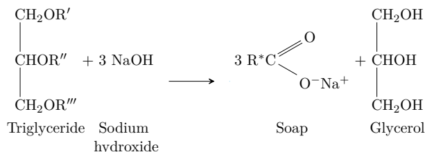
Figure 3.4: Saponification of triglyceride with sodium hydroxide.
