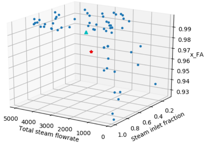
Figure 5.13: Iteration steps for finding the optimal point along the response surface of the fatty acid fraction in the product stream in respect to steam flowrate and inlet fraction (the red point is the final solution of the differential evolution procedure; the triangle is the starting point).
