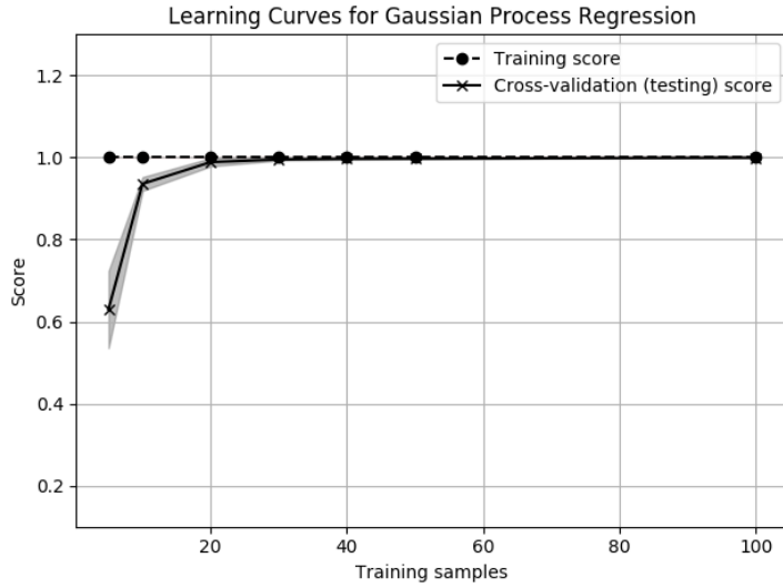
Figure 6.1: Comparison between the behaviour of training score and testing score as a function of the used training samples for Gaussian Process regression of spray column model.
