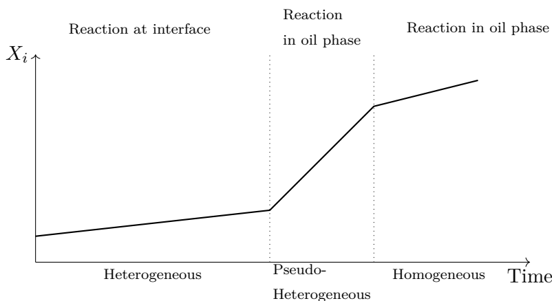
Figure 5.3: Hydrolysis of triglycerides in three step reaction periods ( X_i : conversion of triglyceride i).
