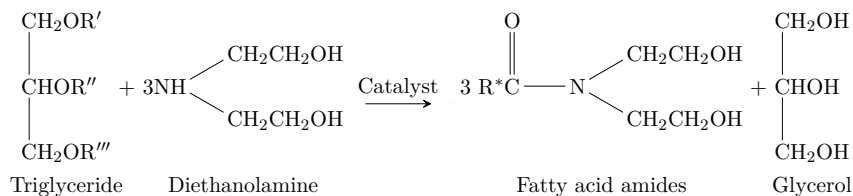
Figure 3.3: Aminolysis of triglyceride with diethanolamine.
