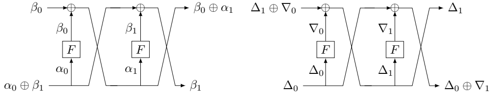
Figure 1: An illustration of how linear approximations/differentials over the F -functions of two consecutive Feistel rounds determine a linear approximation/differential over those rounds.
