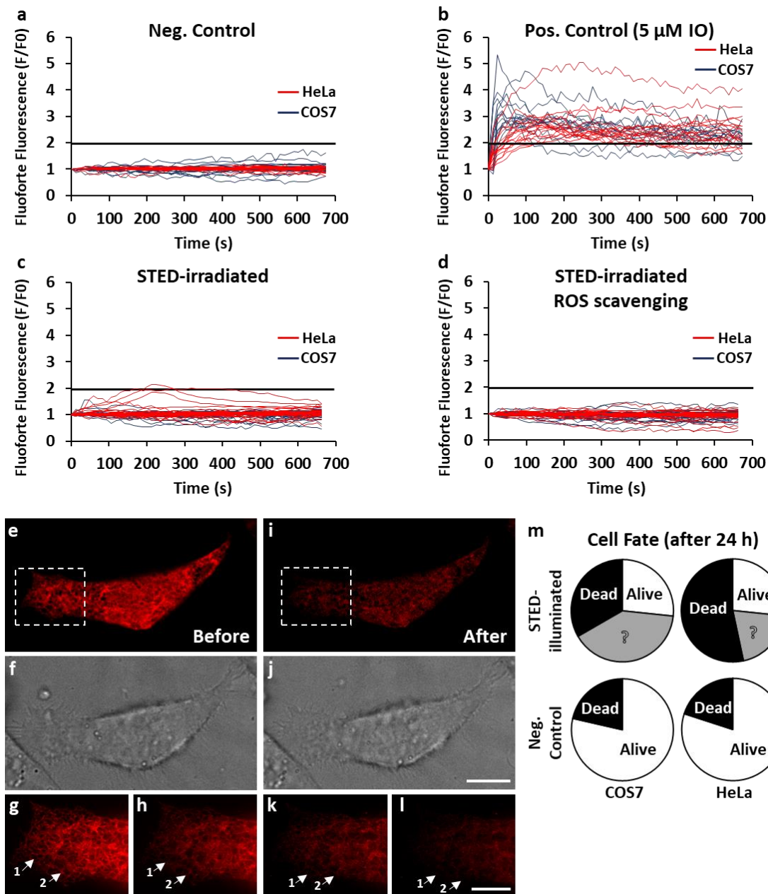
Figure 1 | Short and long-term effects of live-cell STED imaging on COS7 and HeLa cells. (a) Cytoplasmic Ca 2+ -level response of SNAP-Sec61β expressing SiR-labeled cells under negative control conditions (no excitation or STED illumination). (b) Positive control using Ionomycin. (c) STED-irradiated cells using an 8-kHz resonant scanner. (d) STED-irradiated cells with ROS scavenging buffer added. (e-l) Representative fluorescence (e,g-i,k,l) and brightfield (f,j) images of a HeLa cell before and after STED irradiation in ROS scavenging buffer visualizing cell viability via cell morphology and ER movement. Scale bars: 10 μm (j), 5 μm (l). Confocal images (e,i), STED images (g,h,k,l). (m) Long-term viability of STED-irradiated and control cells. Cells are categorized in alive, dead and indeterminable (labeled as “?”; see Supplementary Methods ) after 24 h.
