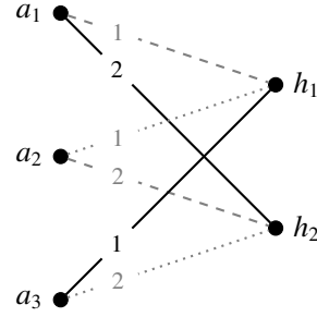
Figure 1: No popular matching exists in this instance. The lists on the left and the numbers on the edges in the figure on the right are the preferences of each applicant. All applicants prefer h_1 to h_2 . The dotted gray matching \{(a_2, h_1), (a_3, h_2)\} is more popular than the dashed gray matching \{(a_1, h_1), (a_2, h_2)\} , because both a_2 and a_3 prefer it. Similarly, the black matching \{(a_1, h_2), (a_3, h_1)\} defeats the dotted gray, and the dashed gray defeats the black.
