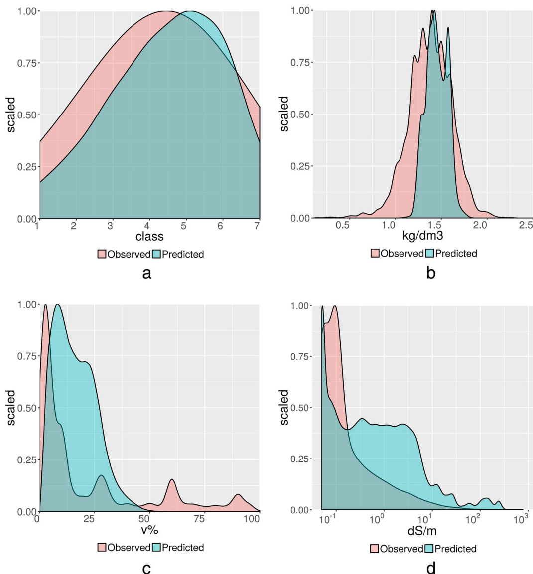
Fig. 3. Scaled probability distributions of observed and predicted soil property values, shown at the back in pink and the front in blue, respectively, for a). drainage class and, aggregated over 150 cm depth, b). bulk density in kg/dm 3 , c). coarse fragments content in v% and d). electric conductivity on a logarithmic scale in dS/m. (For interpretation of the references to colour in this figure legend, the reader is referred to the web version of this article.)
