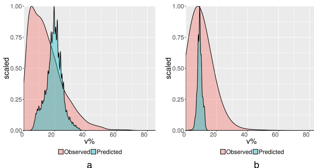
Fig. 5. Scaled probability distributions of observed and mapped (predicted) a). VMC at PWP and b). PAWHC.
