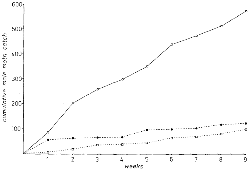
FIG. 1. Cumulative catches of male Chilo partellus moths in traps baited with 437.5 \mu\text{g} (Z)-11-hexadecenal (○—○), 437.5 \mu\text{g} (Z)-11-hexadecenal + 62.5 \mu\text{g} (Z)-11-hexadecen-1-ol (●—●), and 62.5 \mu\text{g} (Z)-11-hexadecen-1-ol (□····□) over 9 weeks (January 20 to March 16, 1977); 5 sites; 1 set of 3 treatments per site; vials renewed weekly.
