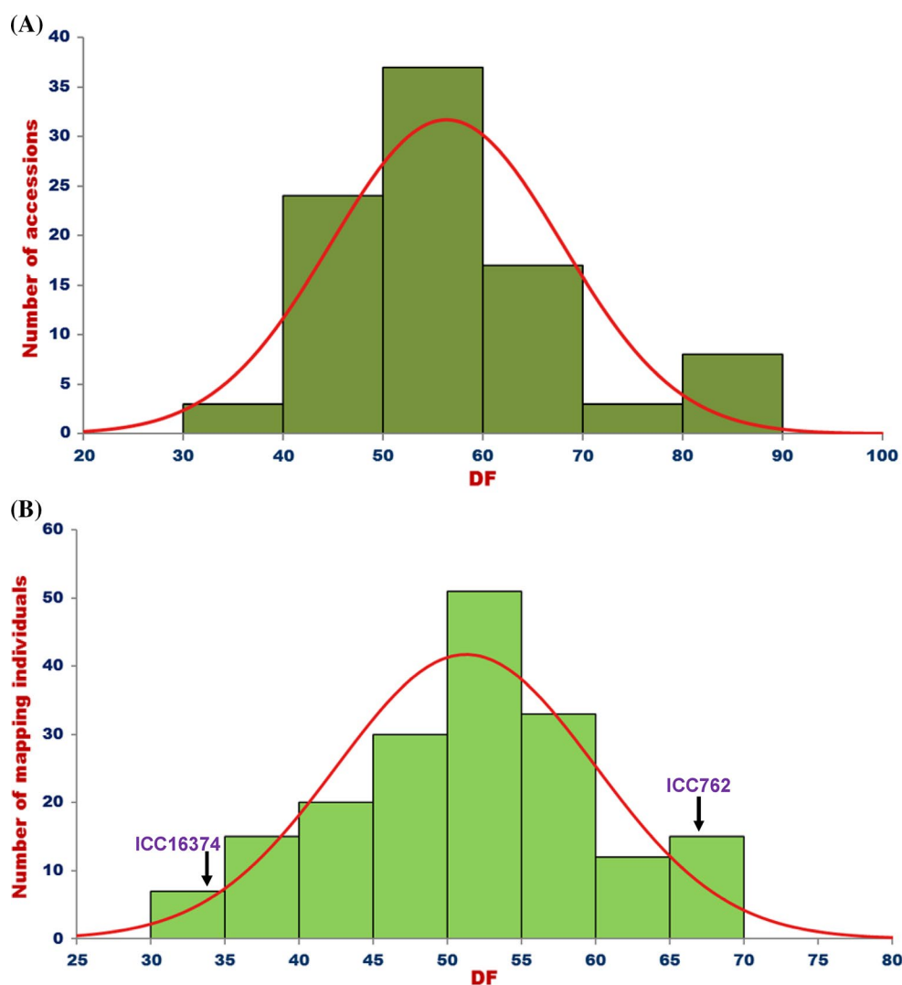
Fig. 3 Frequency distribution of average DF trait variation measured in 92 desi and kabuli chickpea accessions (flowering time association panel A ) as well as in 190 individuals and parental accessions of a F_6 mapping population (ICC 16374 \times ICC 762) B , grown at multi-
