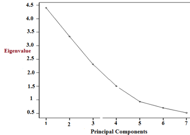
Figure 1. Scree Plot Constructed based on Seven Principal Component and their Eigenvalues
