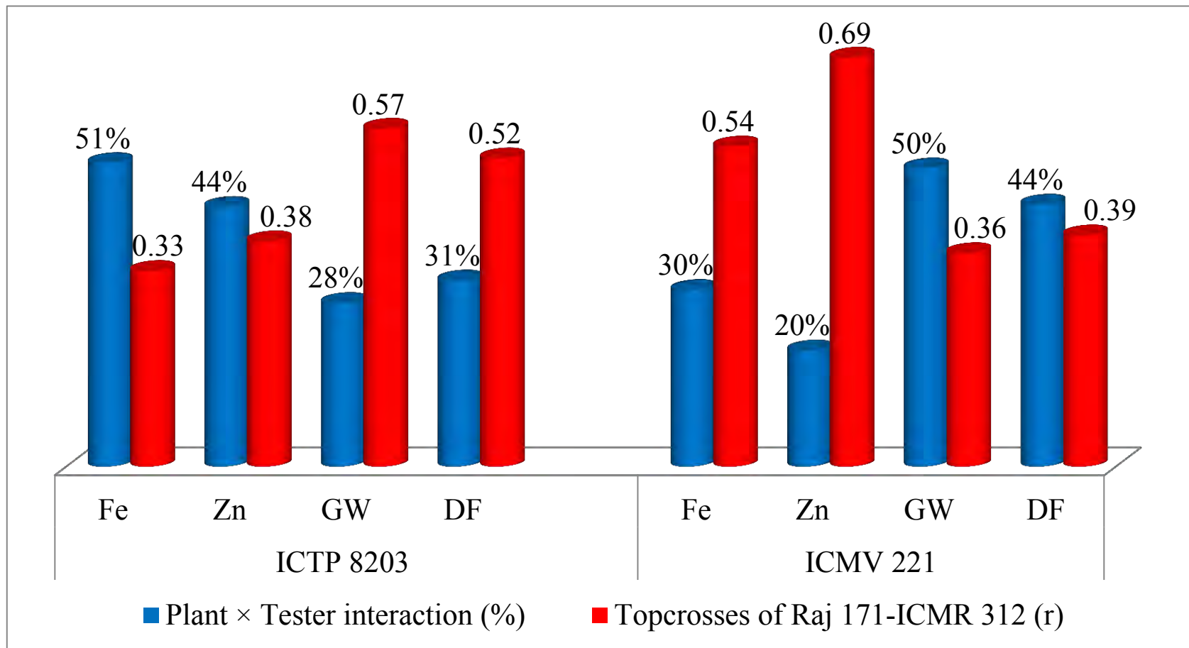
Figure 4.11. Contribution of plant x tester interaction to variability relative to those due to differences among the topcross hybrids of individual plants of ICTP 8203 and ICMV 221 (i.e. P effect), and the correlation between the topcross performance with tester-1 (Raj 171) and tester-2 (ICMR 312) in ICTP 8203 and ICMV 221, averaged over the environments (2012 rainy and 2013 summer seasons), Patancheru
