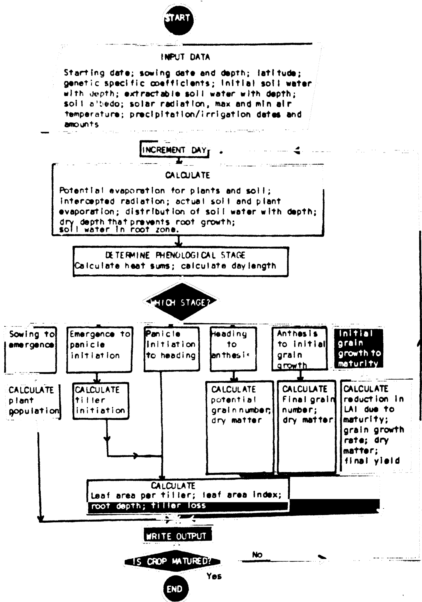
Figure 28. A suggested flow chart for pearl millet growth and development model (after USDA-SEA winter wheat ecological model).
