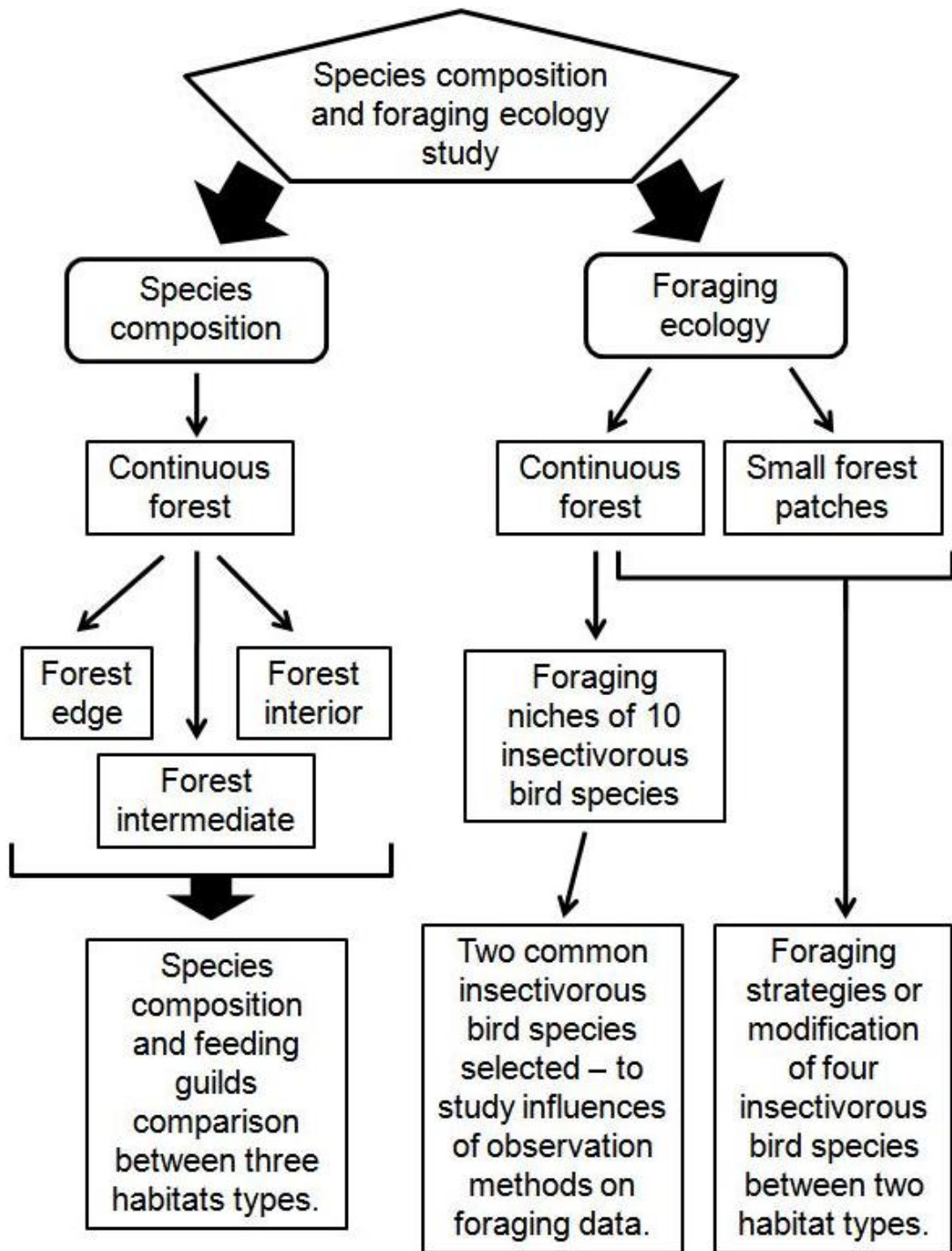
Figure 1.1 Research flow.
