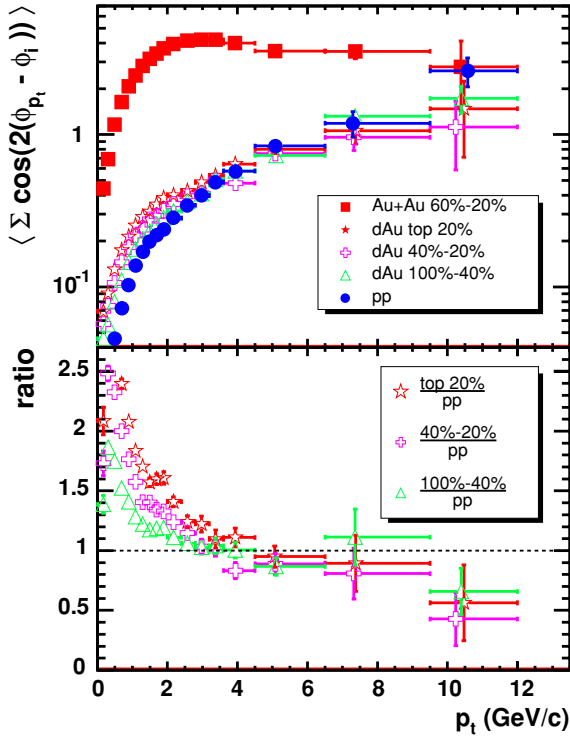
FIG. 13. (Color online) The top panel shows the charged hadron scalar product vs. p_t for different centrality classes in d +Au collisions, and minimum bias p + p collisions. The Au+Au result is put there for a reference. The bottom panel shows the ratio of scalar product from d +Au collisions to minimum bias p + p collisions for three different centrality classes.
