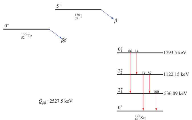
FIG. 2. (Color online) Decay scheme for 130 Te, showing the energy levels (keV) and the branching ratios for the \gamma rays [14].
