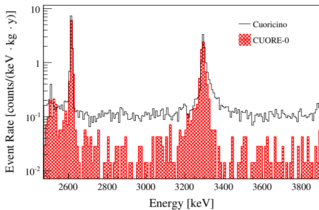
Fig. 4 Background spectrum of CUORE-0 (red with shades) and Cuoricino (black) in the region dominated by degraded \alpha particles. The figure shows reduction of the flat background caused by degraded \alpha particles in the energy region of [2.7–3.1] and [3.4 – 3.9] MeV
