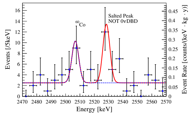
Fig. 3 Blinded energy spectrum and 0\nu\text{DBD} global fit in the region of interest. The unbinned maximum-likelihood fit is shown in solid red line. The dotted blue line illustrates the peak from ^{60}\text{Co} and the linear background only to highlight the difference between salted 0\nu\text{DBD} peak and background. The flat background from the fit is 0.071 \pm 0.011 counts/(keV · kg · y). ^{60}\text{Co} peak position, salted peak position, and rate are 2506.8 \pm 1.1 keV, 2528.4 \pm 1.0 keV, and 1.3 \pm 0.5 counts/(keV · kg · y), respectively
