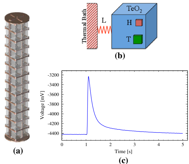
Fig. 1 a CUORE-0 tower array rendering. The tower consists of 13 planes of 4 crystals, mounted in the frame made of copper. b Schematic of a single CUORE-0 bolometer showing the thermistor (T), the heater (H), and the weak thermal link (L) between \text{TeO}_2 crystal and copper thermal bath (not to scale). c An example of a bolometer signal with the energy of approximately 2615 keV. The rise and fall times of this signal are 0.04 s (defined as the time for the pulse amplitude to evolve from 10 to 90 % of its maximum) and 0.26 s (90–30 % of maximum), respectively
