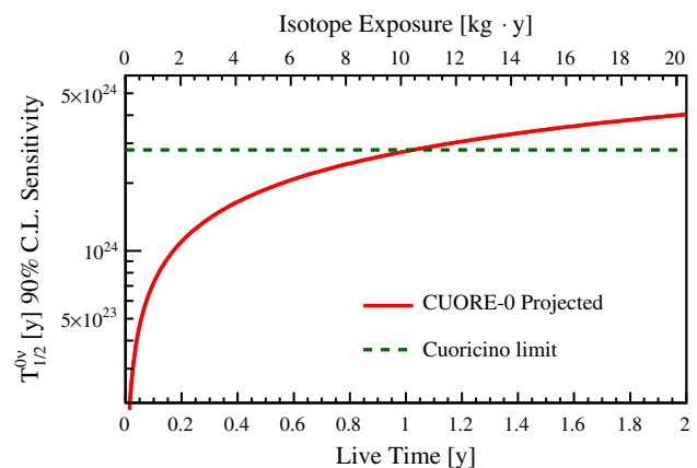
Fig. 5 Sensitivity of CUORE-0 with the measured background rate in the ROI of 0.071 counts/(keV · kg · y) and energy resolution of 5.7 keV FWHM. The CUORE-0 sensitivity is expected to surpass that of Cuoricino with 1 year of live time
