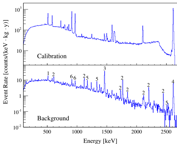
Fig. 2 CUORE-0 calibration ( top panel ) and background spectrum ( bottom panel ) over the data taking period presented in this work. \gamma -ray peaks from known radioactive sources in the background spectrum are labeled as follows: (1) e^+e^- annihilation; (2) ^{214}\text{Bi} ; (3) ^{40}\text{K} ; (4) ^{208}\text{Tl} ; (5) ^{60}\text{Co} ; and (6) ^{228}\text{Ac}
