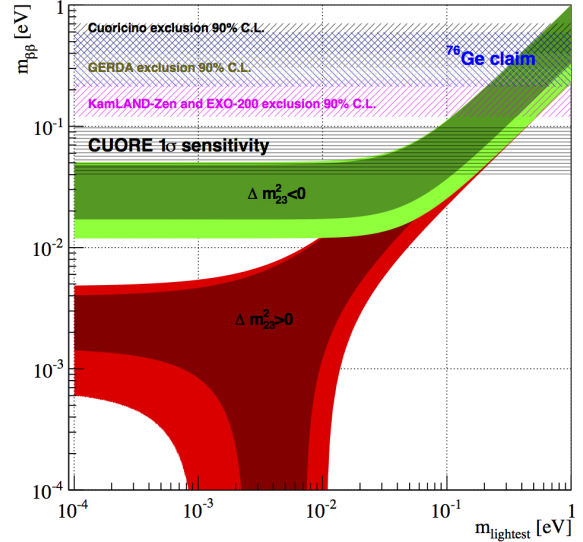
Figure 11. CUORE 1\sigma sensitivity in terms of effective Majorana mass for 5 years live time computed using the experimental parameters given in table 2. The bands corresponds to the maximum and minimum \langle m_{\beta\beta} \rangle values obtained from different nuclear matrix elements.
