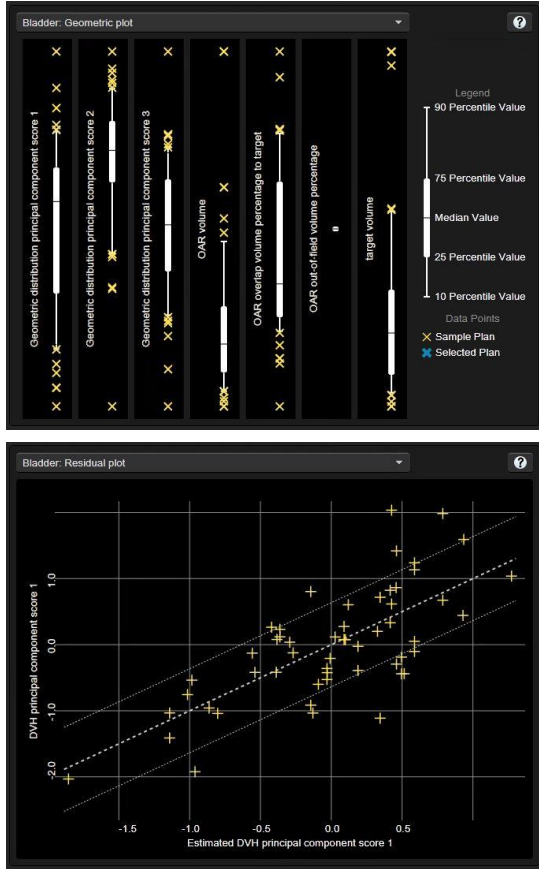
Figure 4: Geometric plots of the bladders used in model training (upper) and the principal component estimation residual plot (lower)
