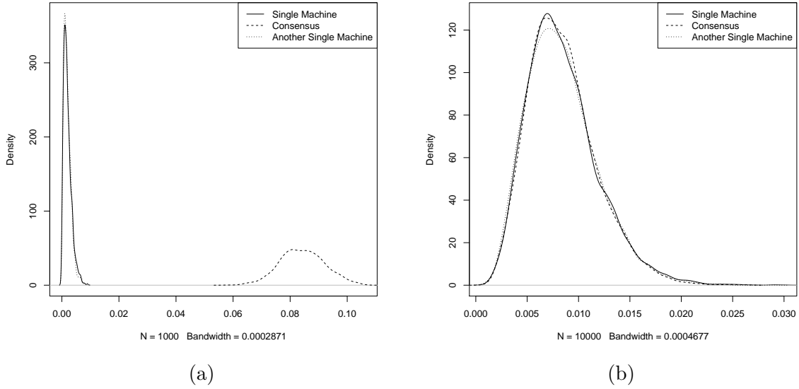
Figure 5: The consensus Monte Carlo distribution (a) performs badly when each worker receives a uniform prior, and (b) performs well with imbalanced shards, when properly weighted.
