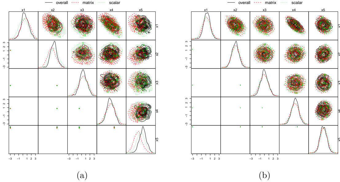
Figure 8: Logistic regression with (a) 1,000 and (b) 10,000 observations per worker. Compare to Figure 7(a). The equal weighting scheme is not shown here, to better focus on matrix and scalar schemes.
